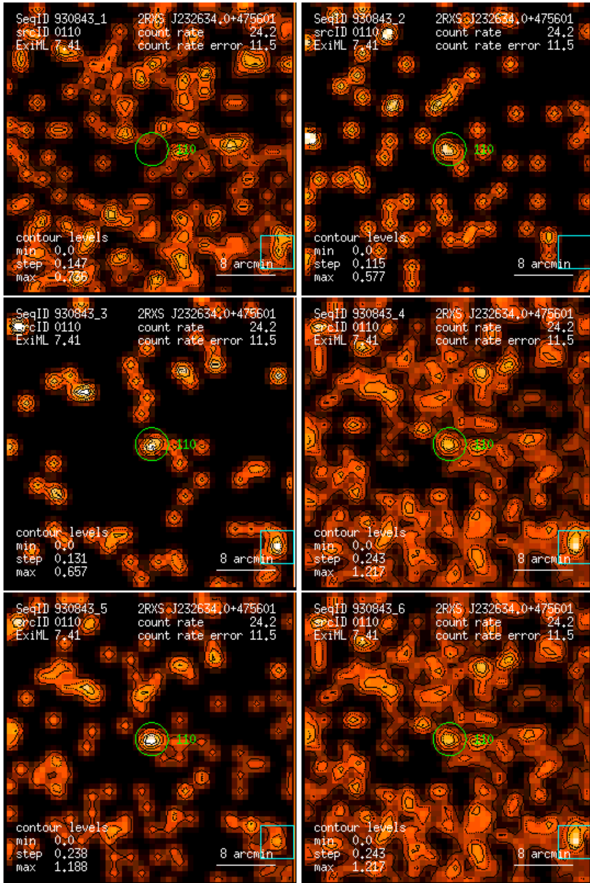
Figure 110: RASS 930843: detection 0110: band rate images, Gaussian filter: (1) PSPC channels 11 – 41, (2) 52 – 90, (3) 91 – 201, (4) 11 – 235, (5) 52 – 201, (6) 11 – 201. Broad band rates in counts/ks. Band rate contour levels in counts/ks/arcmin 2 .
