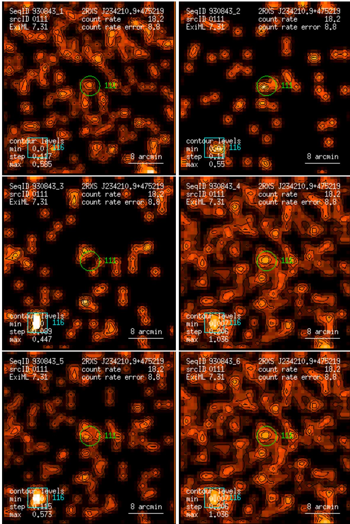
Figure 111: RASS 930843: detection 0111: band rate images, Gaussian filter: (1) PSPC channels 11 – 41, (2) 52 – 90, (3) 91 – 201, (4) 11 – 235, (5) 52 – 201, (6) 11 – 201. Broad band rates in counts/ks. Band rate contour levels in counts/ks/arcmin 2 .
