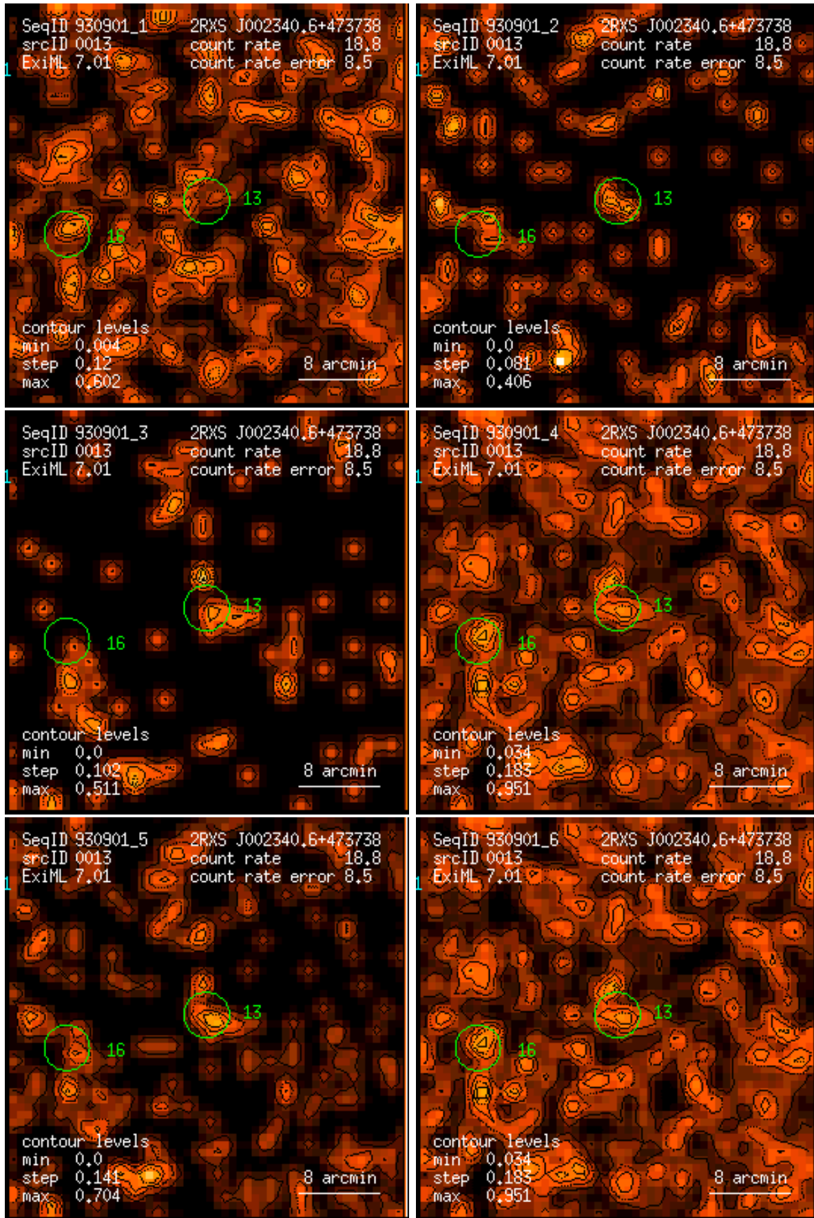
Figure 13: RASS 930901: detection 0013: band rate images, Gaussian filter: (1) PSPC channels 11 – 41, (2) 52 – 90, (3) 91 – 201, (4) 11 – 235, (5) 52 – 201, (6) 11 – 201. Broad band rates in counts/ks. Band rate contour levels in counts/ks/arcmin 2 .
