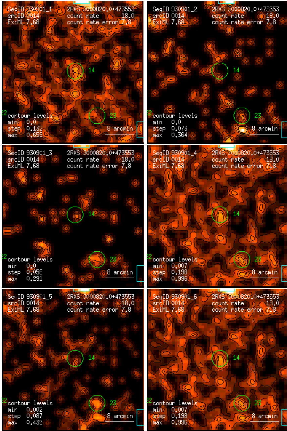
Figure 14: RASS 930901: detection 0014: band rate images, Gaussian filter: (1) PSPC channels 11 – 41, (2) 52 – 90, (3) 91 – 201, (4) 11 – 235, (5) 52 – 201, (6) 11 – 201. Broad band rates in counts/ks. Band rate contour levels in counts/ks/arcmin 2 .
