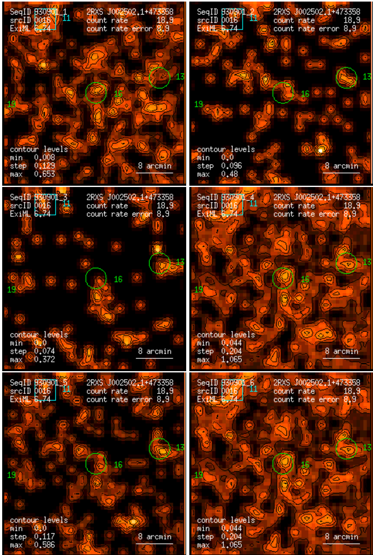
Figure 16: RASS 930901: detection 0016: band rate images, Gaussian filter: (1) PSPC channels 11 – 41, (2) 52 – 90, (3) 91 – 201, (4) 11 – 235, (5) 52 – 201, (6) 11 – 201. Broad band rates in counts/ks. Band rate contour levels in counts/ks/arcmin 2 .
