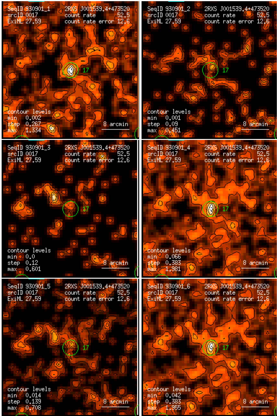
Figure 17: RASS 930901: detection 0017: band rate images, Gaussian filter: (1) PSPC channels 11 – 41, (2) 52 – 90, (3) 91 – 201, (4) 11 – 235, (5) 52 – 201, (6) 11 – 201. Broad band rates in counts/ks. Band rate contour levels in counts/ks/arcmin 2 .
