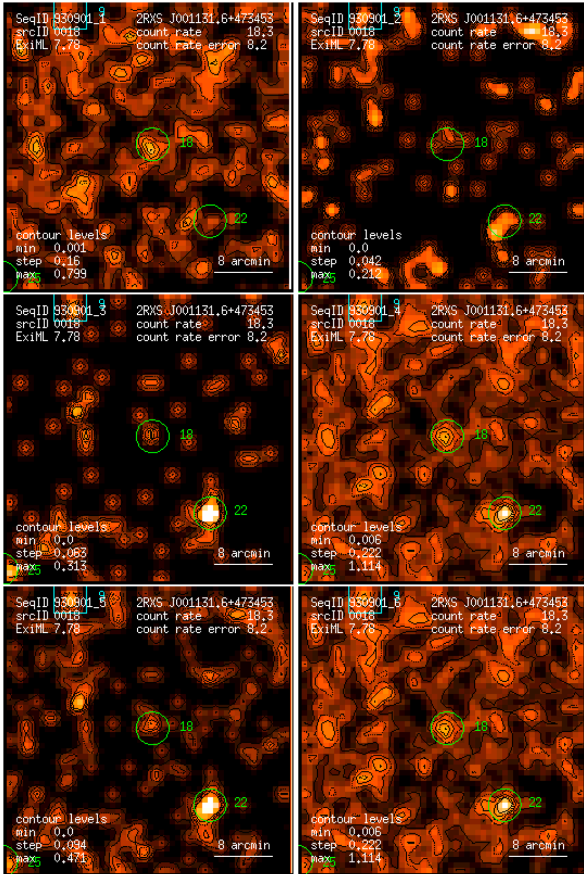
Figure 18: RASS 930901: detection 0018: band rate images, Gaussian filter: (1) PSPC channels 11 – 41, (2) 52 – 90, (3) 91 – 201, (4) 11 – 235, (5) 52 – 201, (6) 11 – 201. Broad band rates in counts/ks. Band rate contour levels in counts/ks/arcmin 2 .
