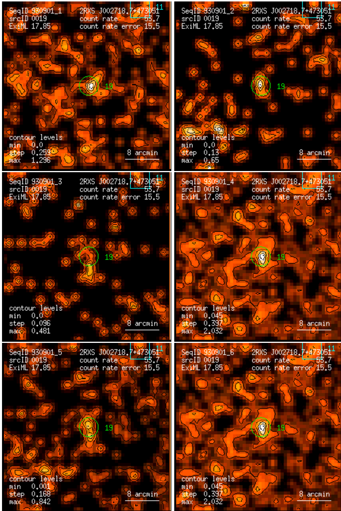
Figure 19: RASS 930901: detection 0019: band rate images, Gaussian filter: (1) PSPC channels 11 – 41, (2) 52 – 90, (3) 91 – 201, (4) 11 – 235, (5) 52 – 201, (6) 11 – 201. Broad band rates in counts/ks. Band rate contour levels in counts/ks/arcmin 2 .
