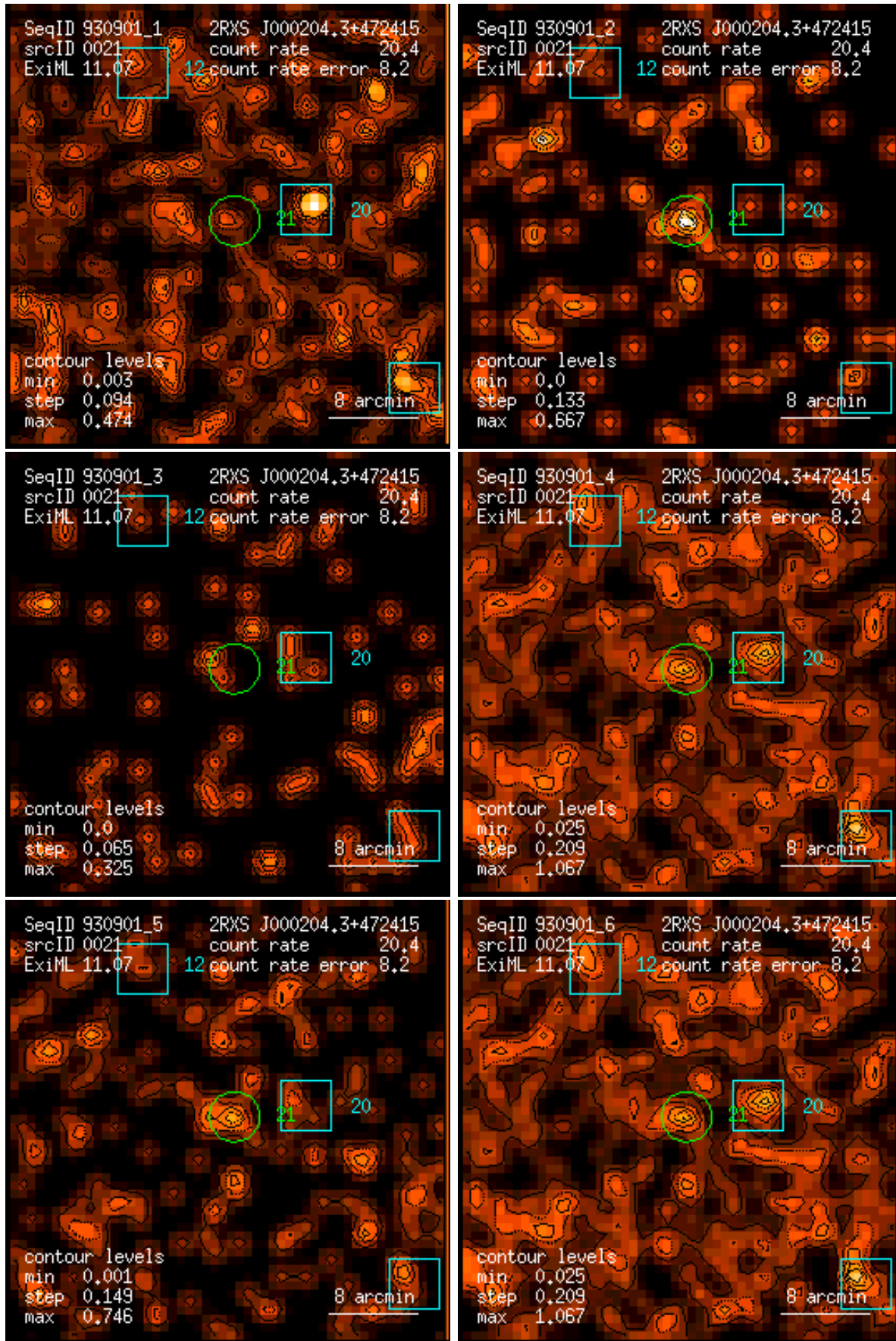
Figure 21: RASS 930901: detection 0021: band rate images, Gaussian filter: (1) PSPC channels 11 – 41, (2) 52 – 90, (3) 91 – 201, (4) 11 – 235, (5) 52 – 201, (6) 11 – 201. Broad band rates in counts/ks. Band rate contour levels in counts/ks/arcmin 2 .
