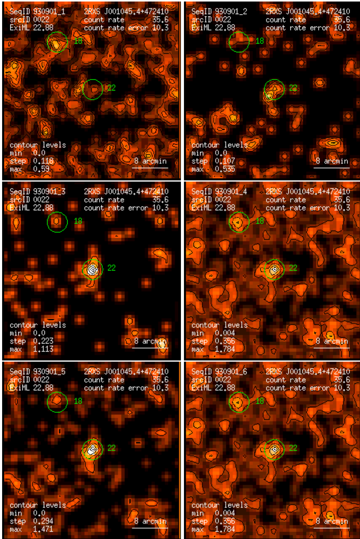
Figure 22: RASS 930901: detection 0022: band rate images, Gaussian filter: (1) PSPC channels 11 – 41, (2) 52 – 90, (3) 91 – 201, (4) 11 – 235, (5) 52 – 201, (6) 11 – 201. Broad band rates in counts/ks. Band rate contour levels in counts/ks/arcmin 2 .
