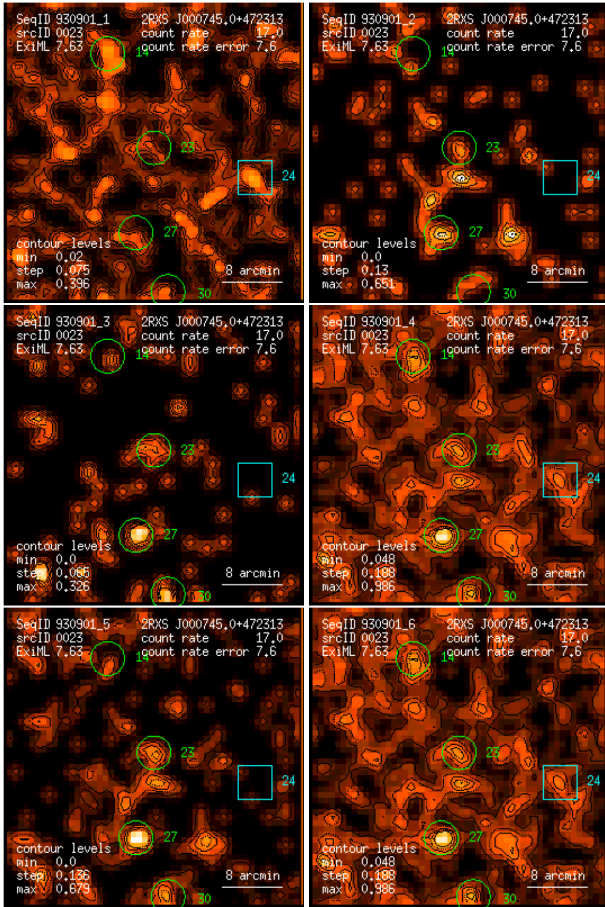
Figure 23: RASS 930901: detection 0023: band rate images, Gaussian filter: (1) PSPC channels 11 – 41, (2) 52 – 90, (3) 91 – 201, (4) 11 – 235, (5) 52 – 201, (6) 11 – 201. Broad band rates in counts/ks. Band rate contour levels in counts/ks/arcmin 2 .
