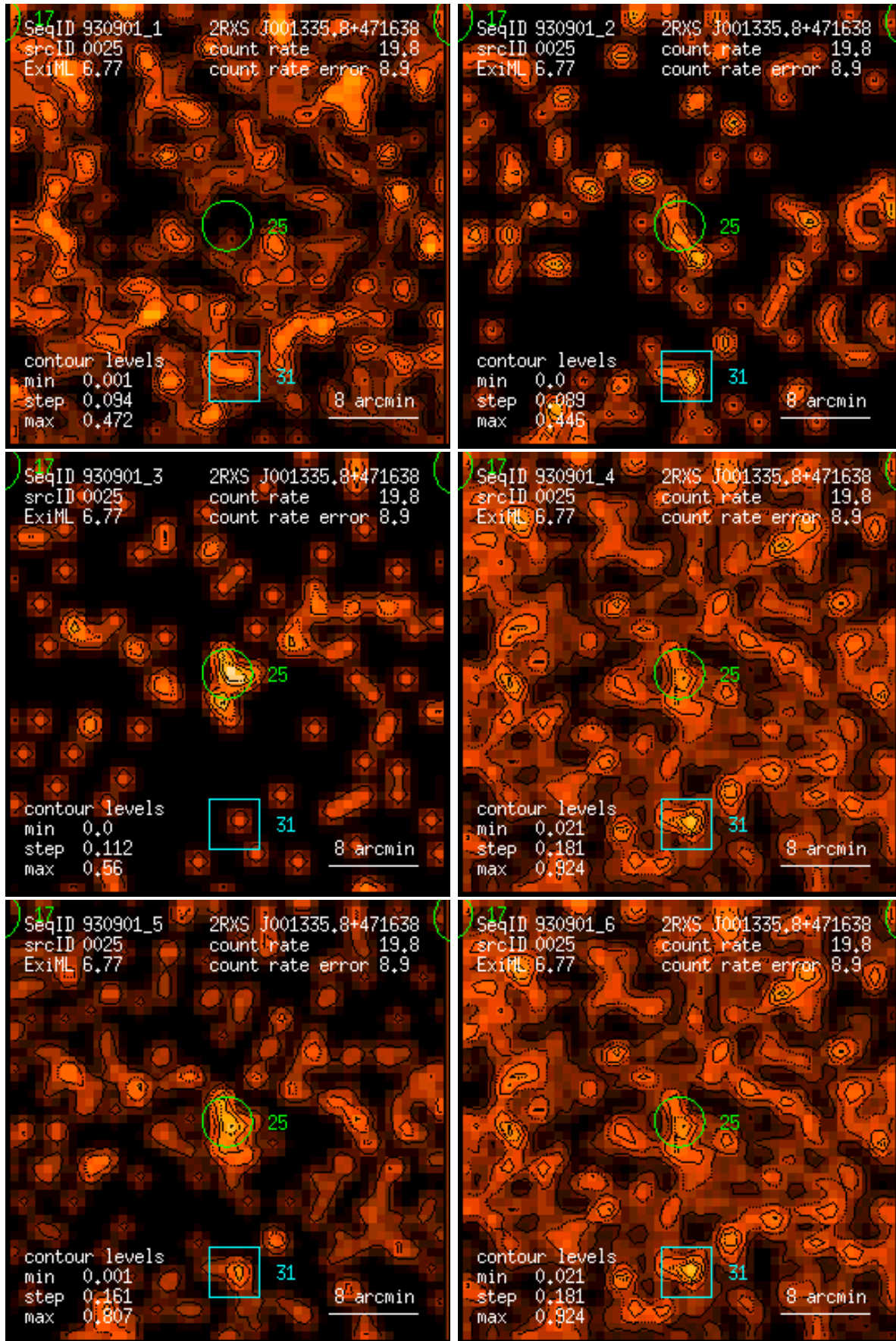
Figure 25: RASS 930901: detection 0025: band rate images, Gaussian filter: (1) PSPC channels 11 – 41, (2) 52 – 90, (3) 91 – 201, (4) 11 – 235, (5) 52 – 201, (6) 11 – 201. Broad band rates in counts/ks. Band rate contour levels in counts/ks/arcmin 2 .
