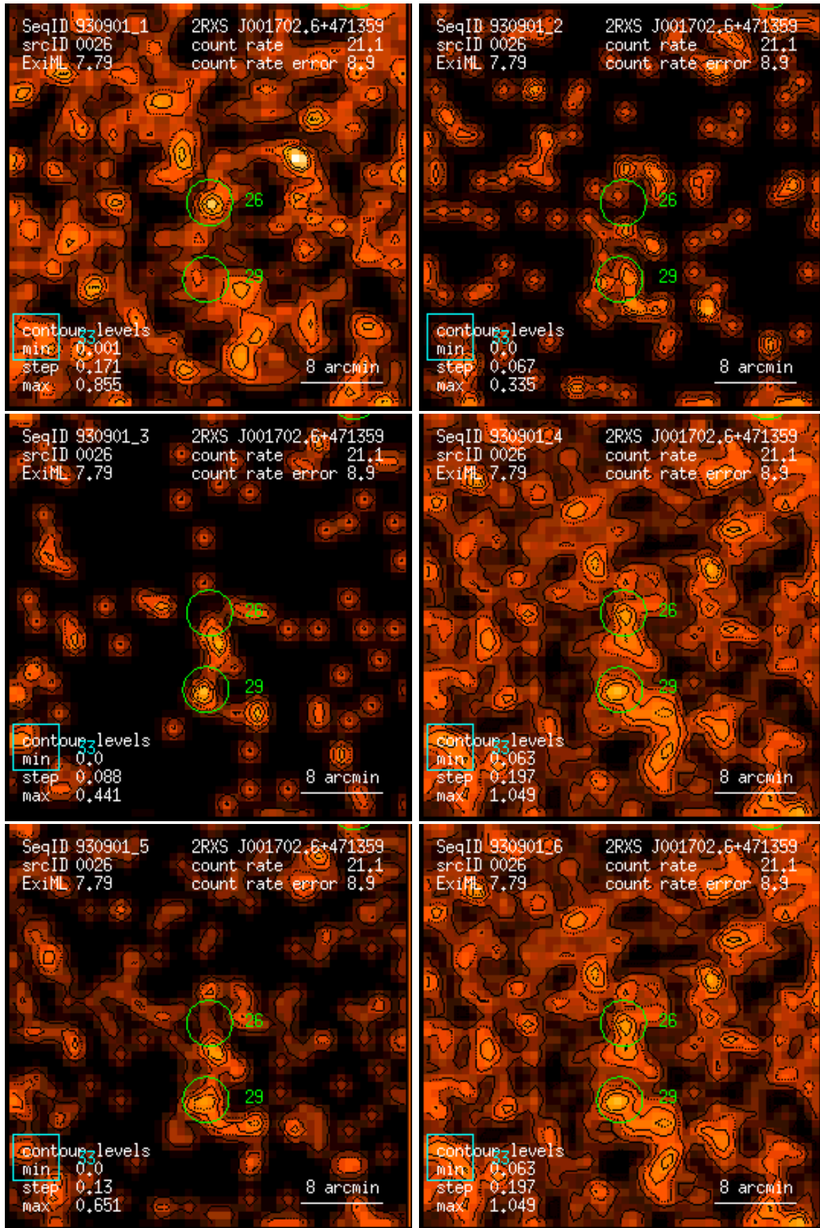
Figure 26: RASS 930901: detection 0026: band rate images, Gaussian filter: (1) PSPC channels 11 – 41, (2) 52 – 90, (3) 91 – 201, (4) 11 – 235, (5) 52 – 201, (6) 11 – 201. Broad band rates in counts/ks. Band rate contour levels in counts/ks/arcmin 2 .
