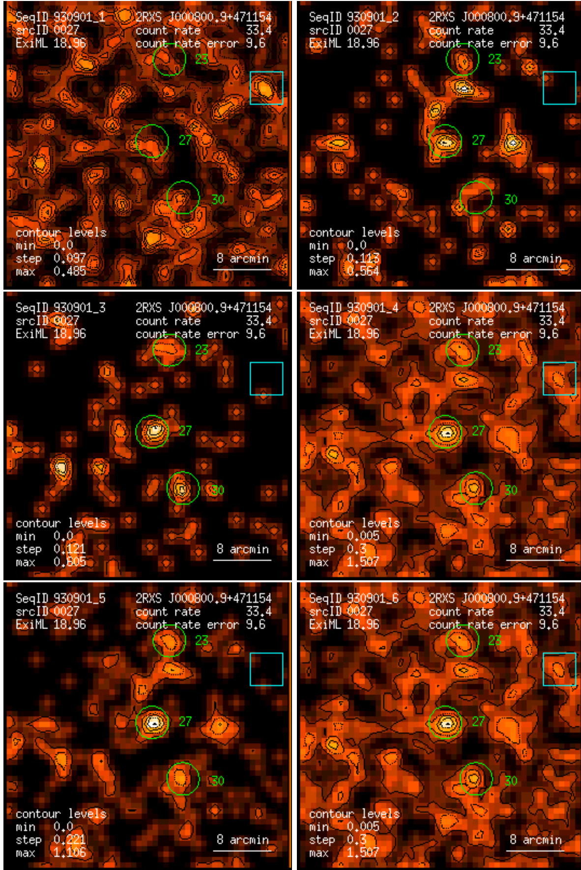
Figure 27: RASS 930901: detection 0027: band rate images, Gaussian filter: (1) PSPC channels 11 – 41, (2) 52 – 90, (3) 91 – 201, (4) 11 – 235, (5) 52 – 201, (6) 11 – 201. Broad band rates in counts/ks. Band rate contour levels in counts/ks/arcmin 2 .
