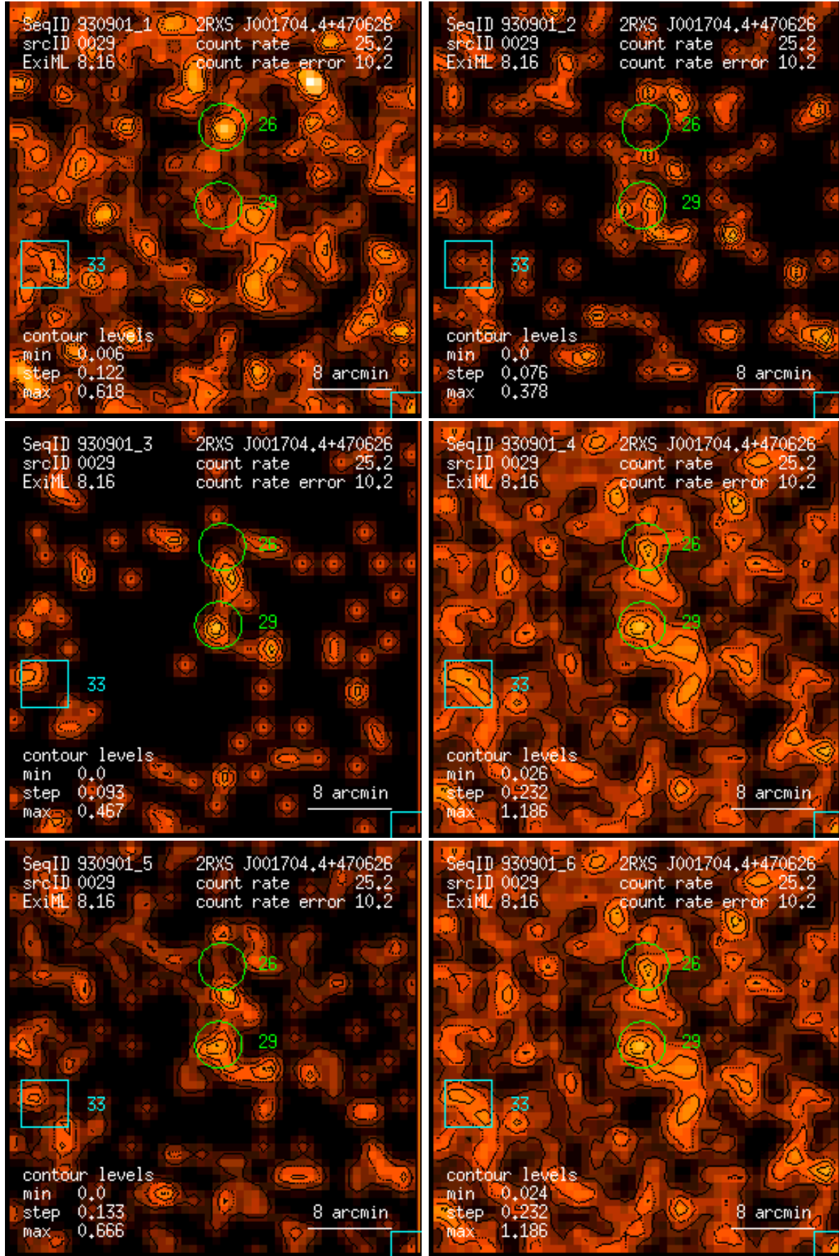
Figure 29: RASS 930901: detection 0029: band rate images, Gaussian filter: (1) PSPC channels 11 – 41, (2) 52 – 90, (3) 91 – 201, (4) 11 – 235, (5) 52 – 201, (6) 11 – 201. Broad band rates in counts/ks. Band rate contour levels in counts/ks/arcmin 2 .
