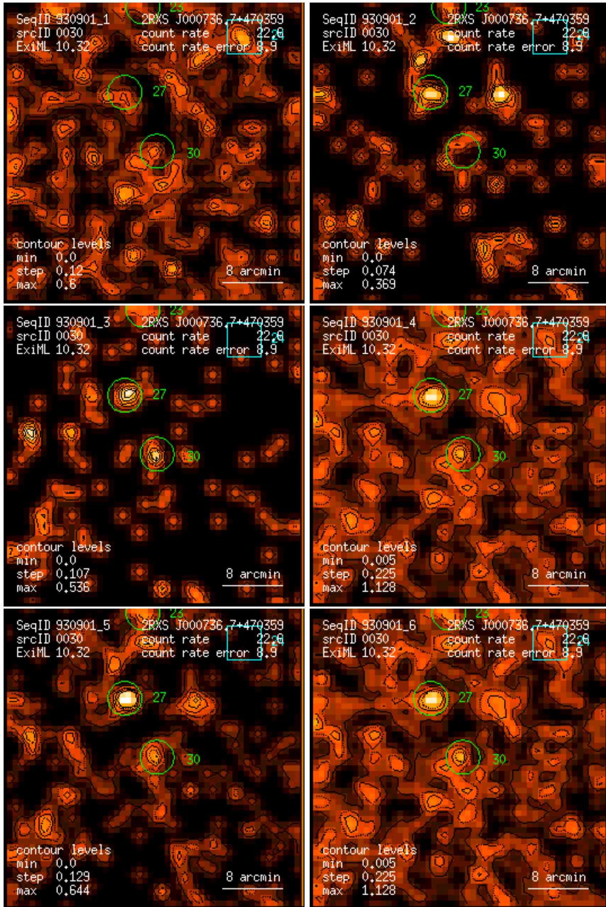
Figure 30: RASS 930901: detection 0030: band rate images, Gaussian filter: (1) PSPC channels 11 – 41, (2) 52 – 90, (3) 91 – 201, (4) 11 – 235, (5) 52 – 201, (6) 11 – 201. Broad band rates in counts/ks. Band rate contour levels in counts/ks/arcmin 2 .
