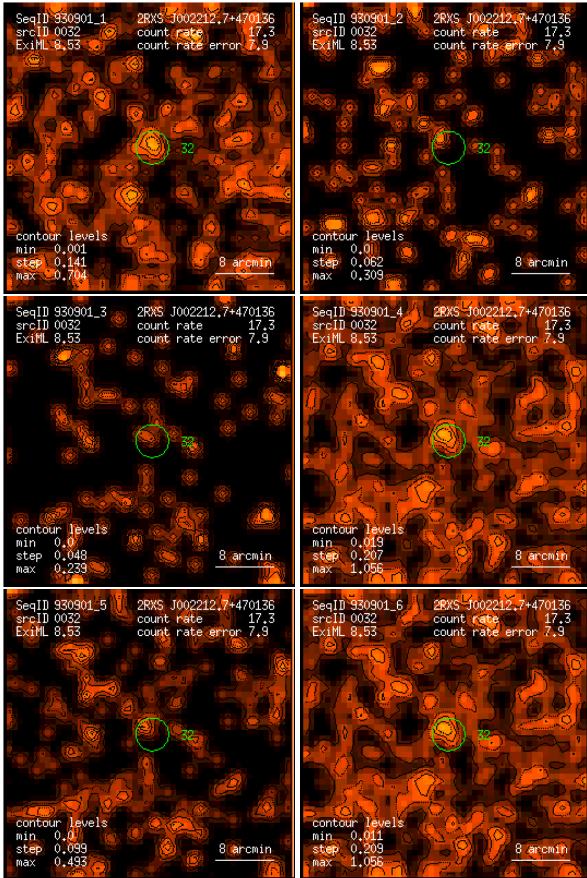
Figure 32: RASS 930901: detection 0032: band rate images, Gaussian filter: (1) PSPC channels 11 – 41, (2) 52 – 90, (3) 91 – 201, (4) 11 – 235, (5) 52 – 201, (6) 11 – 201. Broad band rates in counts/ks. Band rate contour levels in counts/ks/arcmin 2 .
