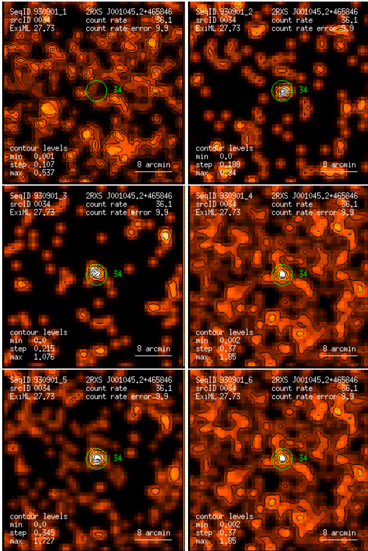
Figure 34: RASS 930901: detection 0034: band rate images, Gaussian filter: (1) PSPC channels 11 – 41, (2) 52 – 90, (3) 91 – 201, (4) 11 – 235, (5) 52 – 201, (6) 11 – 201. Broad band rates in counts/ks. Band rate contour levels in counts/ks/arcmin 2 .
