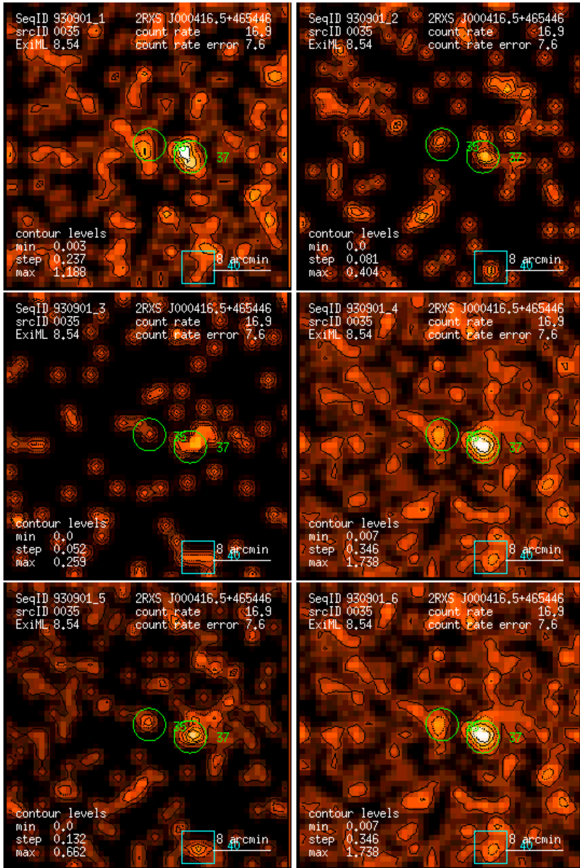
Figure 35: RASS 930901: detection 0035: band rate images, Gaussian filter: (1) PSPC channels 11 – 41, (2) 52 – 90, (3) 91 – 201, (4) 11 – 235, (5) 52 – 201, (6) 11 – 201. Broad band rates in counts/ks. Band rate contour levels in counts/ks/arcmin 2 .
