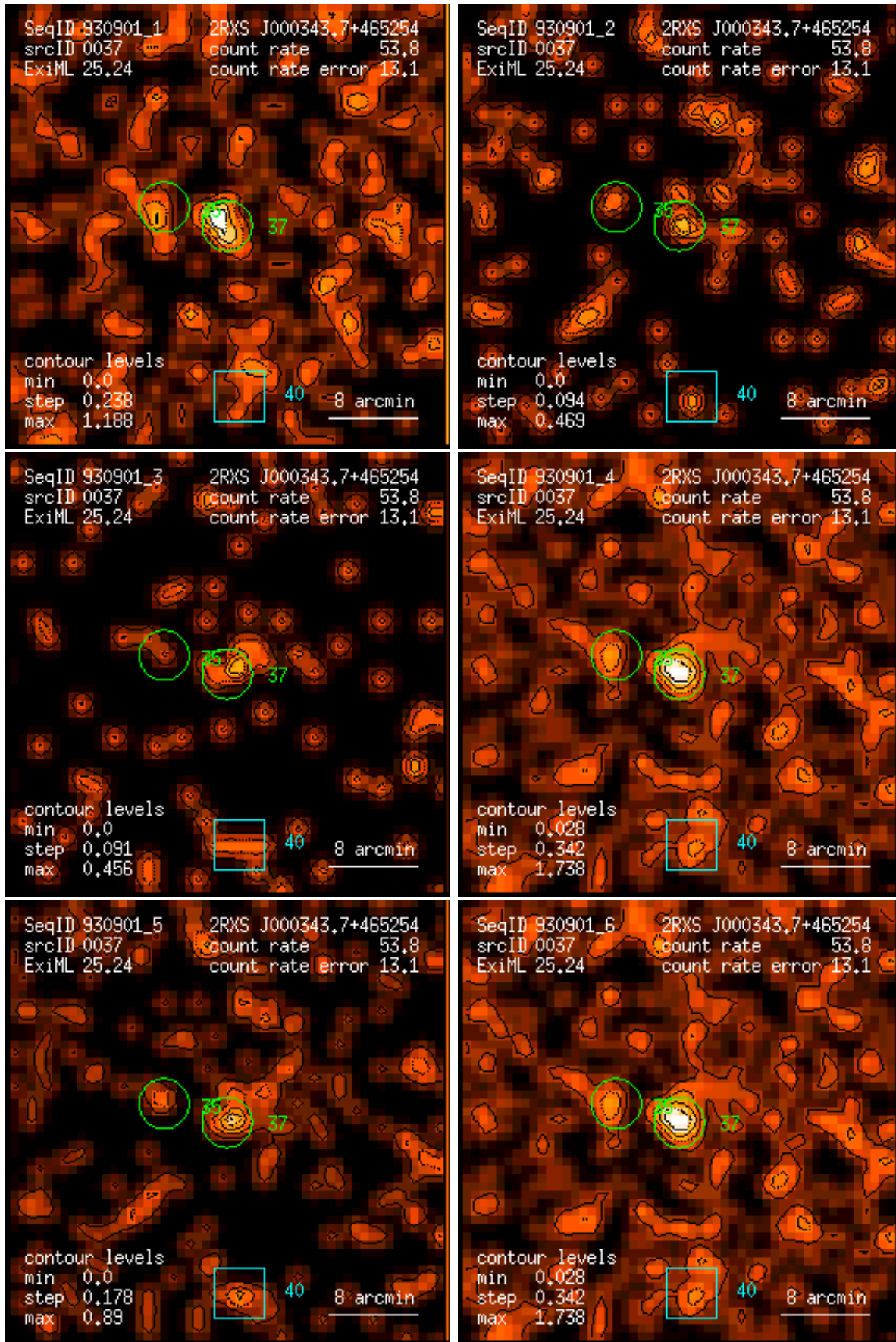
Figure 37: RASS 930901: detection 0037: band rate images, Gaussian filter: (1) PSPC channels 11 – 41, (2) 52 – 90, (3) 91 – 201, (4) 11 – 235, (5) 52 – 201, (6) 11 – 201. Broad band rates in counts/ks. Band rate contour levels in counts/ks/arcmin 2 .
