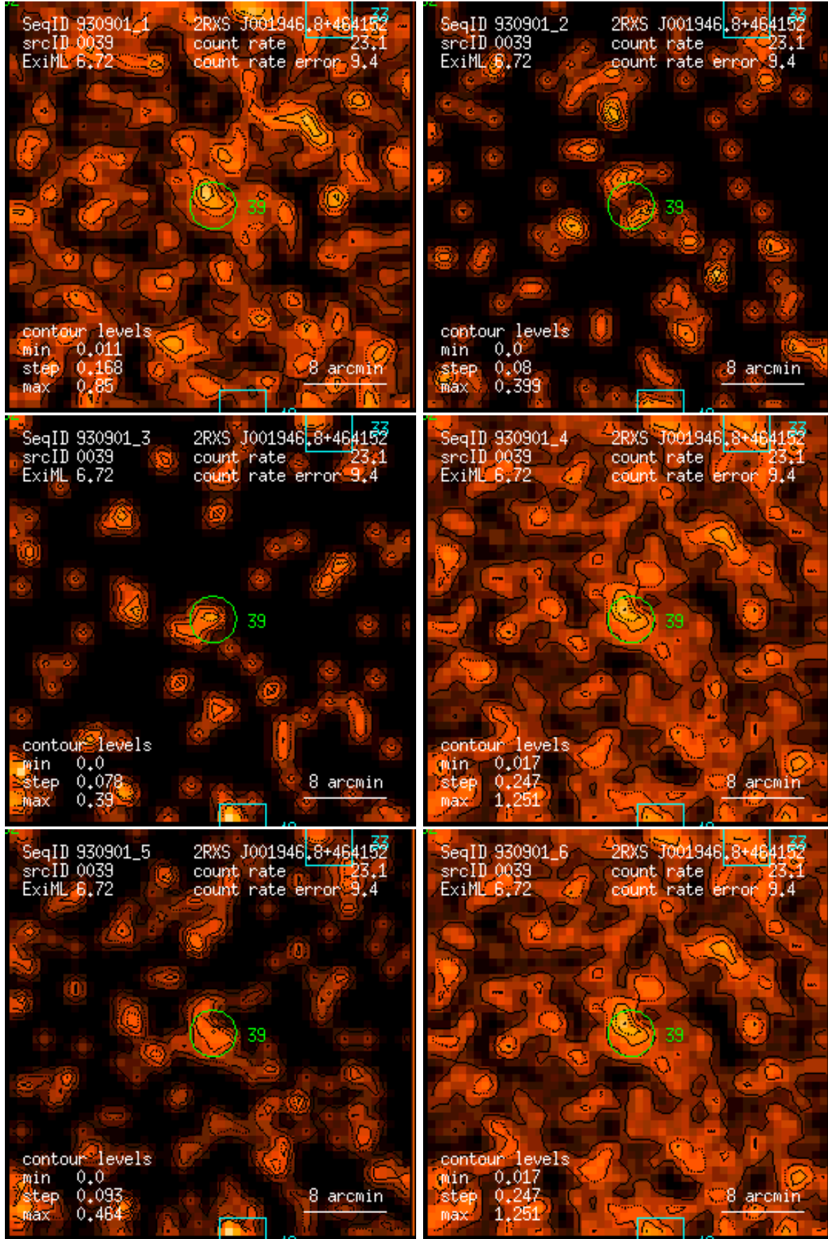
Figure 39: RASS 930901: detection 0039: band rate images, Gaussian filter: (1) PSPC channels 11 – 41, (2) 52 – 90, (3) 91 – 201, (4) 11 – 235, (5) 52 – 201, (6) 11 – 201. Broad band rates in counts/ks. Band rate contour levels in counts/ks/arcmin 2 .
