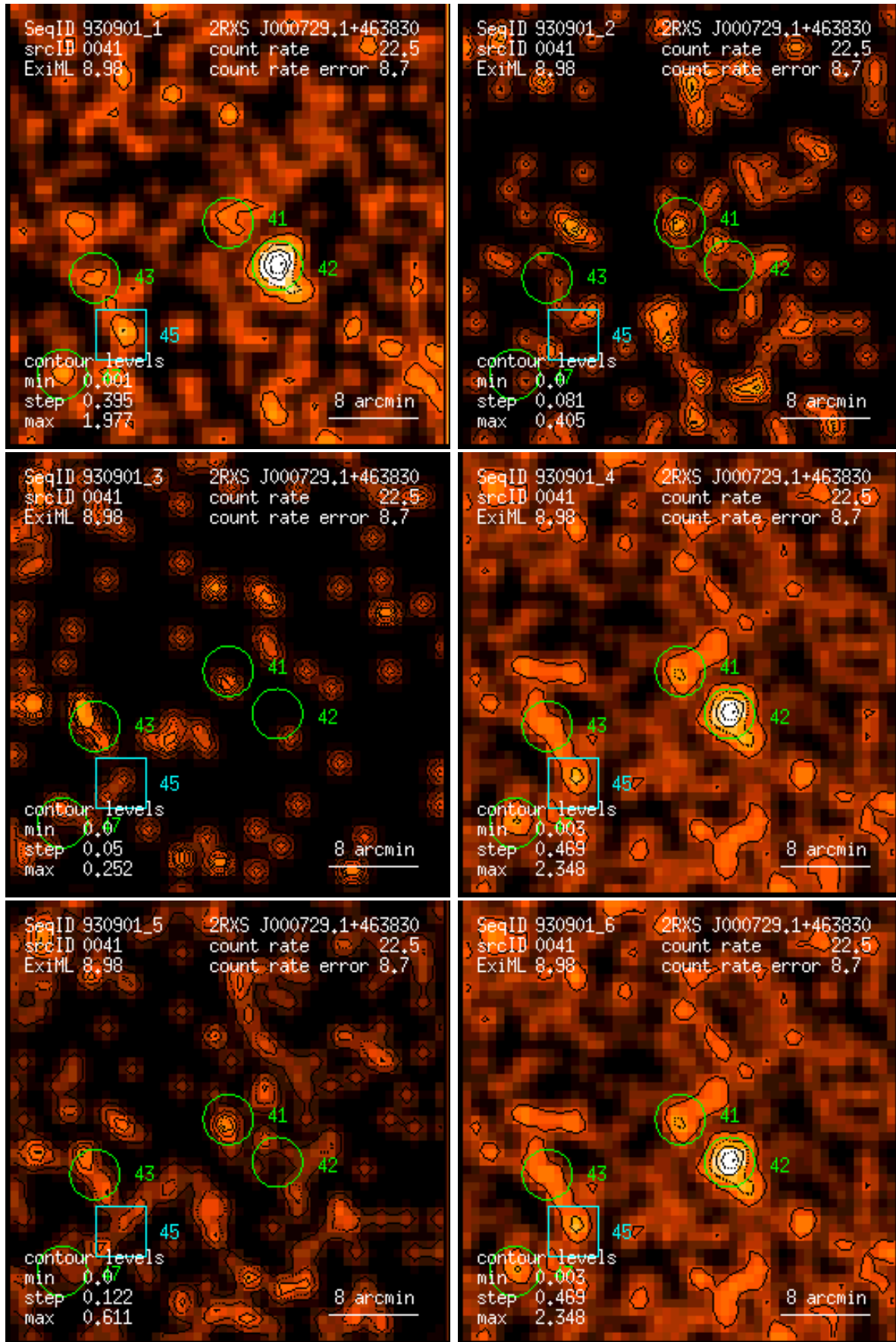
Figure 41: RASS 930901: detection 0041: band rate images, Gaussian filter: (1) PSPC channels 11 – 41, (2) 52 – 90, (3) 91 – 201, (4) 11 – 235, (5) 52 – 201, (6) 11 – 201. Broad band rates in counts/ks. Band rate contour levels in counts/ks/arcmin 2 .
