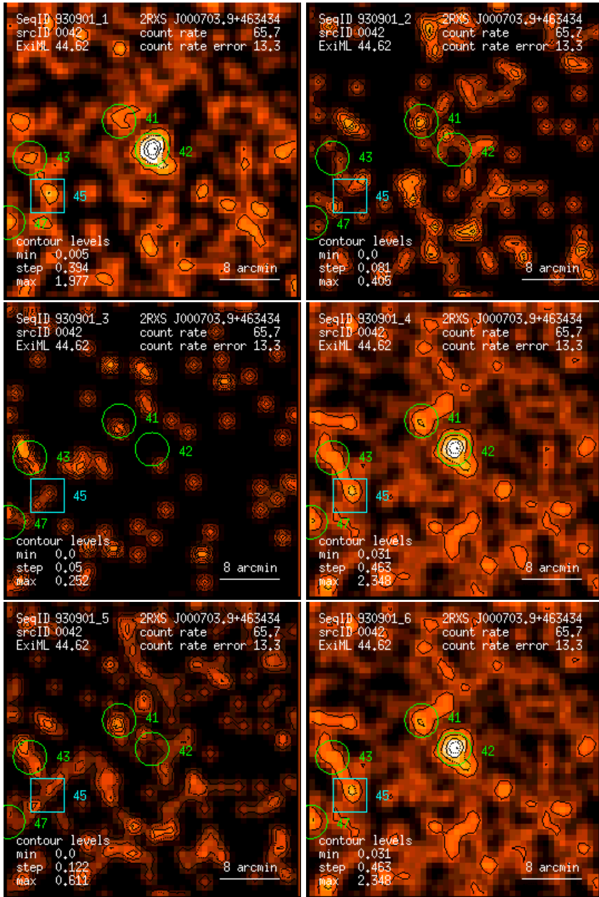
Figure 42: RASS 930901: detection 0042: band rate images, Gaussian filter: (1) PSPC channels 11 – 41, (2) 52 – 90, (3) 91 – 201, (4) 11 – 235, (5) 52 – 201, (6) 11 – 201. Broad band rates in counts/ks. Band rate contour levels in counts/ks/arcmin 2 .
