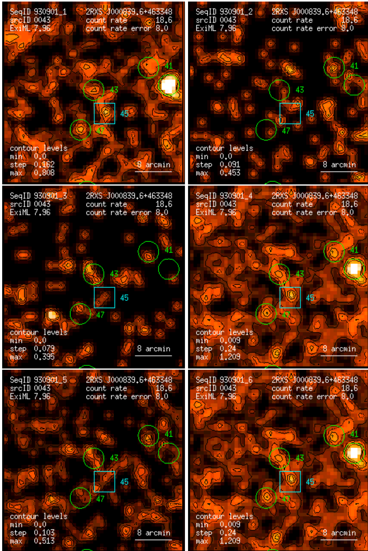
Figure 43: RASS 930901: detection 0043: band rate images, Gaussian filter: (1) PSPC channels 11 – 41, (2) 52 – 90, (3) 91 – 201, (4) 11 – 235, (5) 52 – 201, (6) 11 – 201. Broad band rates in counts/ks. Band rate contour levels in counts/ks/arcmin 2 .
