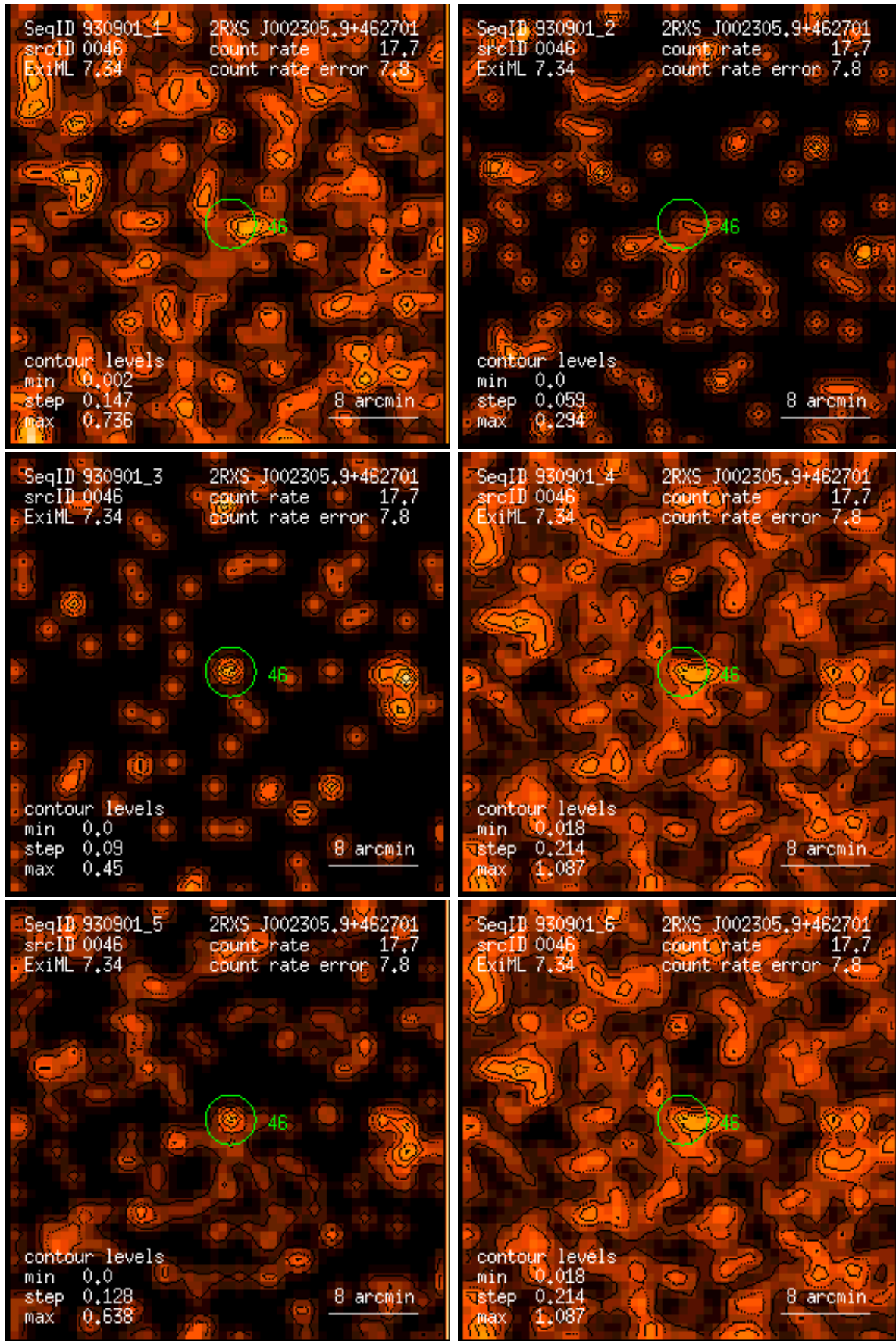
Figure 46: RASS 930901: detection 0046: band rate images, Gaussian filter: (1) PSPC channels 11 – 41, (2) 52 – 90, (3) 91 – 201, (4) 11 – 235, (5) 52 – 201, (6) 11 – 201. Broad band rates in counts/ks. Band rate contour levels in counts/ks/arcmin 2 .
