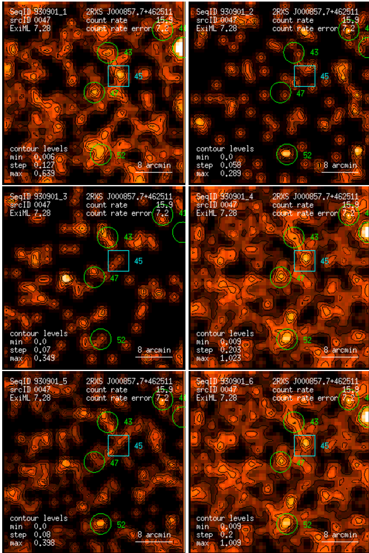
Figure 47: RASS 930901: detection 0047: band rate images, Gaussian filter: (1) PSPC channels 11 – 41, (2) 52 – 90, (3) 91 – 201, (4) 11 – 235, (5) 52 – 201, (6) 11 – 201. Broad band rates in counts/ks. Band rate contour levels in counts/ks/arcmin 2 .
