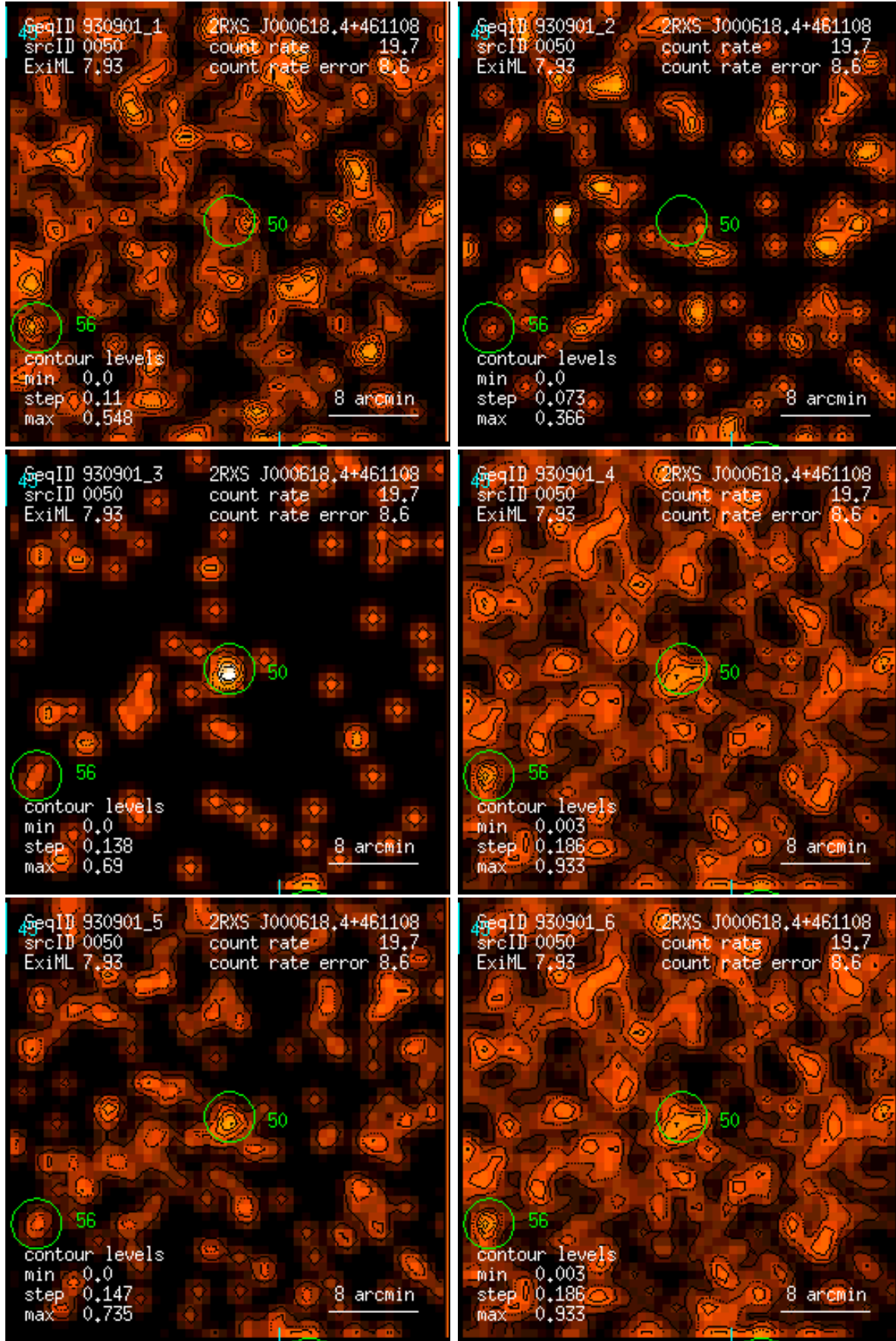
Figure 50: RASS 930901: detection 0050: band rate images, Gaussian filter: (1) PSPC channels 11 – 41, (2) 52 – 90, (3) 91 – 201, (4) 11 – 235, (5) 52 – 201, (6) 11 – 201. Broad band rates in counts/ks. Band rate contour levels in counts/ks/arcmin 2 .
