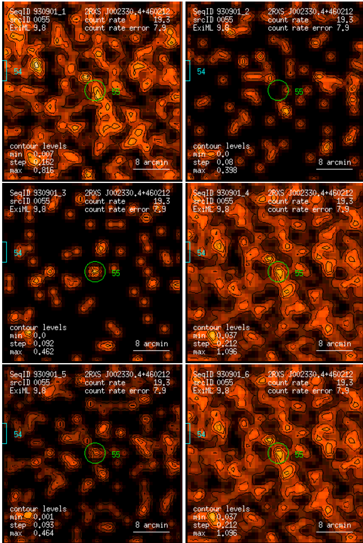
Figure 55: RASS 930901: detection 0055: band rate images, Gaussian filter: (1) PSPC channels 11 – 41, (2) 52 – 90, (3) 91 – 201, (4) 11 – 235, (5) 52 – 201, (6) 11 – 201. Broad band rates in counts/ks. Band rate contour levels in counts/ks/arcmin 2 .
