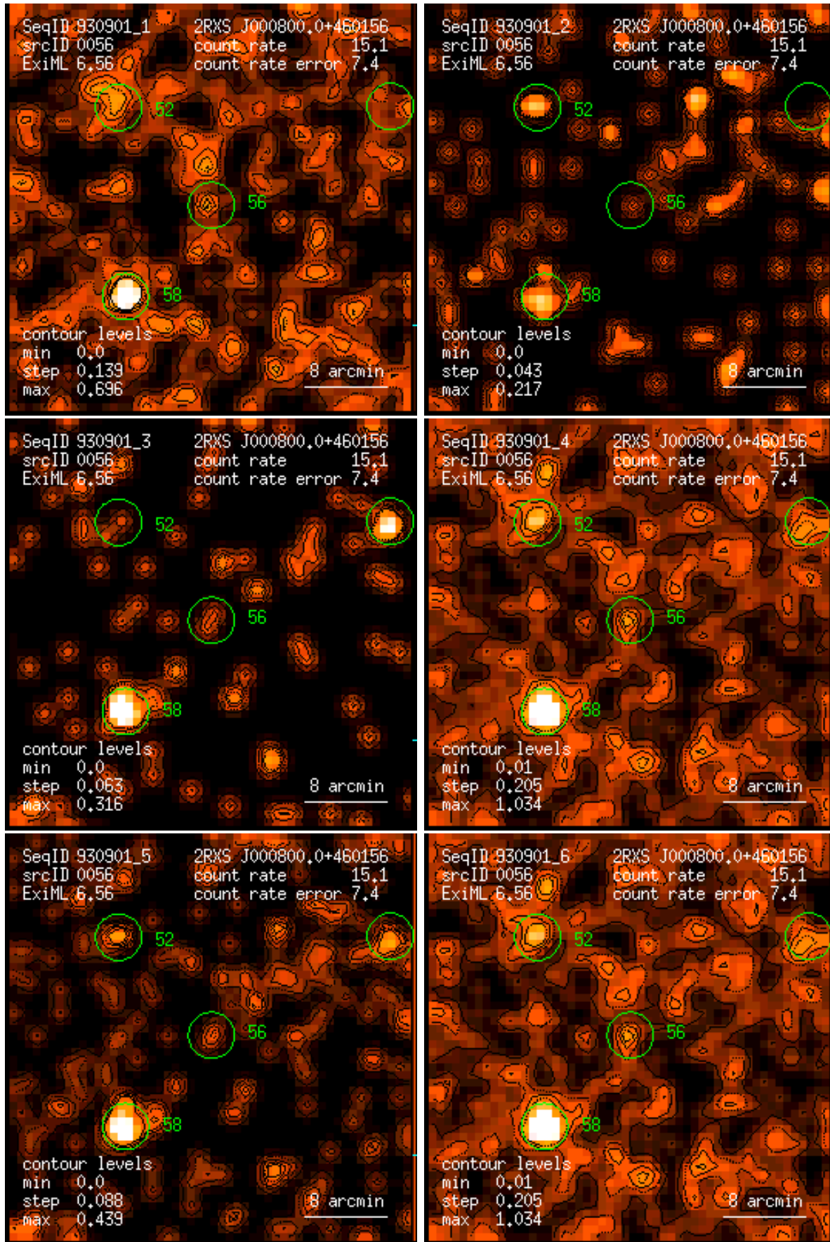
Figure 56: RASS 930901: detection 0056: band rate images, Gaussian filter: (1) PSPC channels 11 – 41, (2) 52 – 90, (3) 91 – 201, (4) 11 – 235, (5) 52 – 201, (6) 11 – 201. Broad band rates in counts/ks. Band rate contour levels in counts/ks/arcmin 2 .
