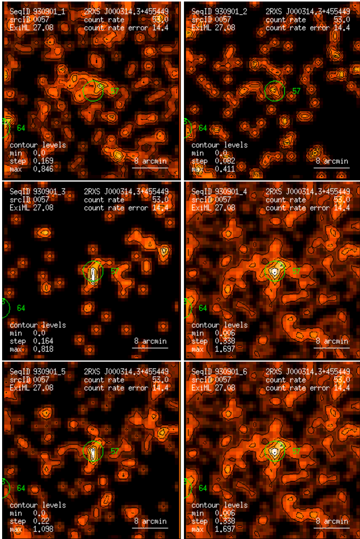
Figure 57: RASS 930901: detection 0057: band rate images, Gaussian filter: (1) PSPC channels 11 – 41, (2) 52 – 90, (3) 91 – 201, (4) 11 – 235, (5) 52 – 201, (6) 11 – 201. Broad band rates in counts/ks. Band rate contour levels in counts/ks/arcmin 2 .
