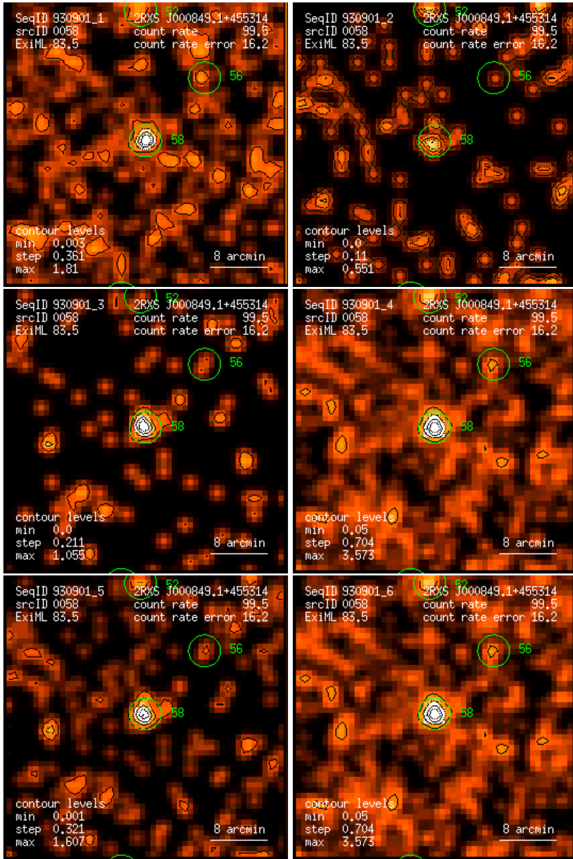
Figure 58: RASS 930901: detection 0058: band rate images, Gaussian filter: (1) PSPC channels 11 – 41, (2) 52 – 90, (3) 91 – 201, (4) 11 – 235, (5) 52 – 201, (6) 11 – 201. Broad band rates in counts/ks. Band rate contour levels in counts/ks/arcmin 2 .
