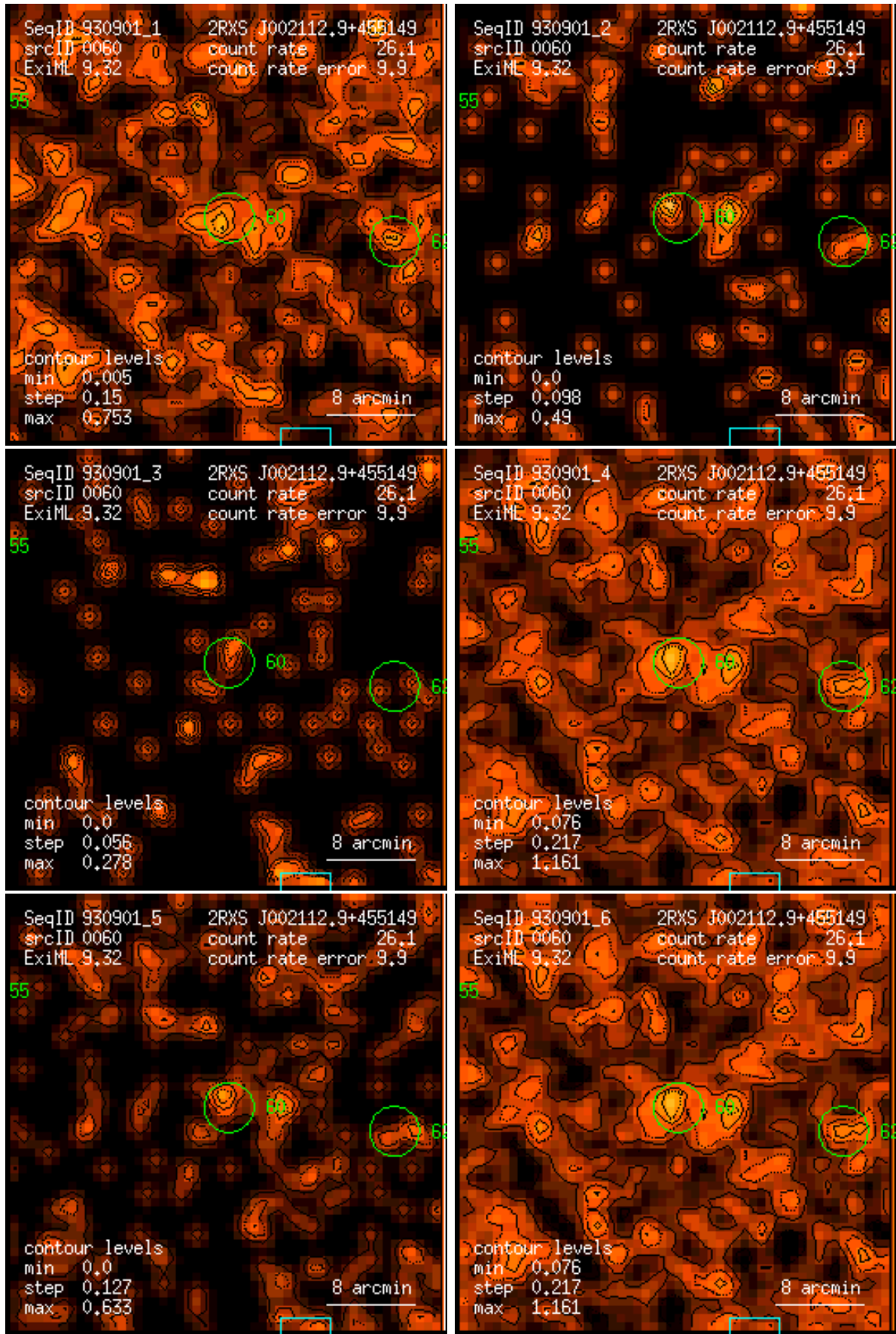
Figure 60: RASS 930901: detection 0060: band rate images, Gaussian filter: (1) PSPC channels 11 – 41, (2) 52 – 90, (3) 91 – 201, (4) 11 – 235, (5) 52 – 201, (6) 11 – 201. Broad band rates in counts/ks. Band rate contour levels in counts/ks/arcmin 2 .
