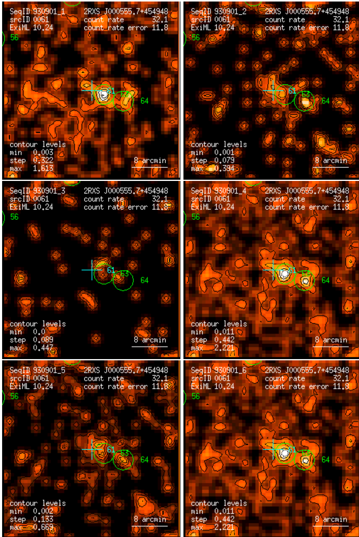
Figure 61: RASS 930901: detection 0061: band rate images, Gaussian filter: (1) PSPC channels 11 – 41, (2) 52 – 90, (3) 91 – 201, (4) 11 – 235, (5) 52 – 201, (6) 11 – 201. Broad band rates in counts/ks. Band rate contour levels in counts/ks/arcmin 2 .
