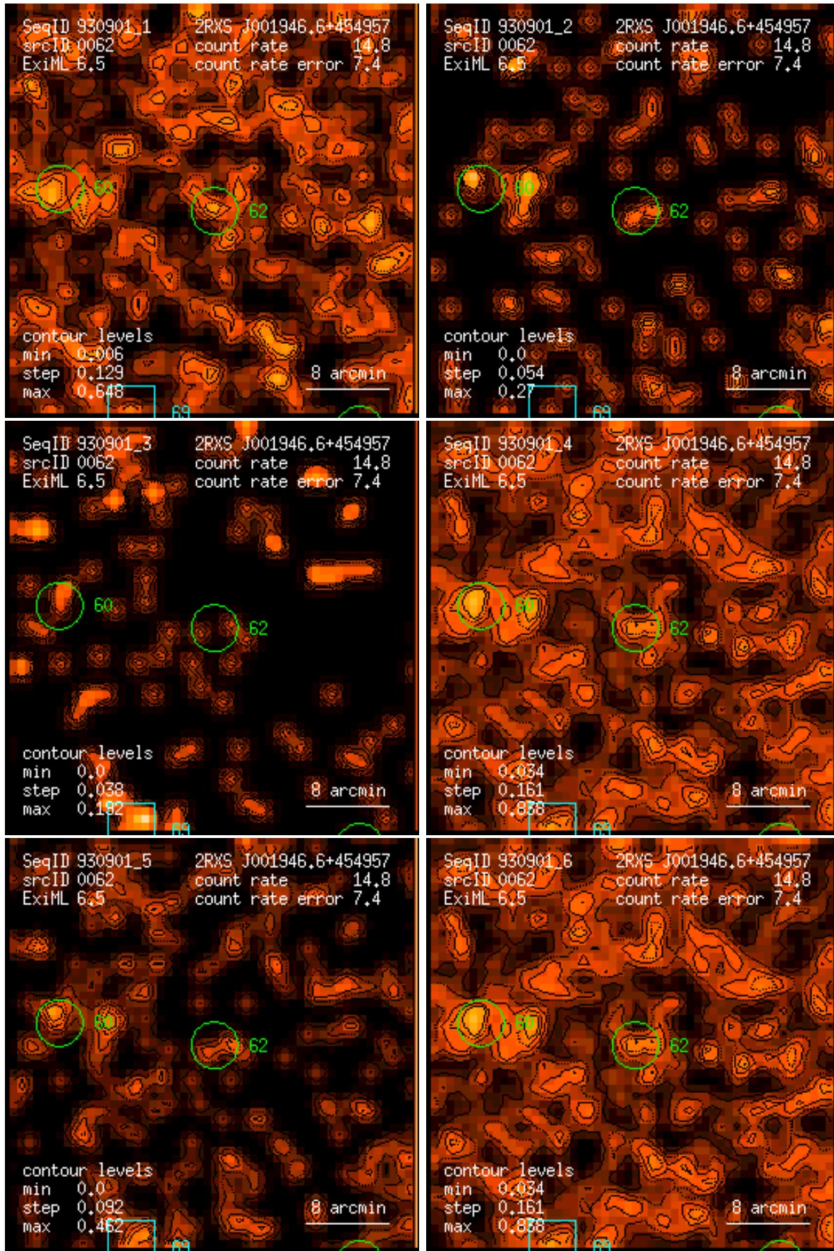
Figure 62: RASS 930901: detection 0062: band rate images, Gaussian filter: (1) PSPC channels 11 – 41, (2) 52 – 90, (3) 91 – 201, (4) 11 – 235, (5) 52 – 201, (6) 11 – 201. Broad band rates in counts/ks. Band rate contour levels in counts/ks/arcmin 2 .
