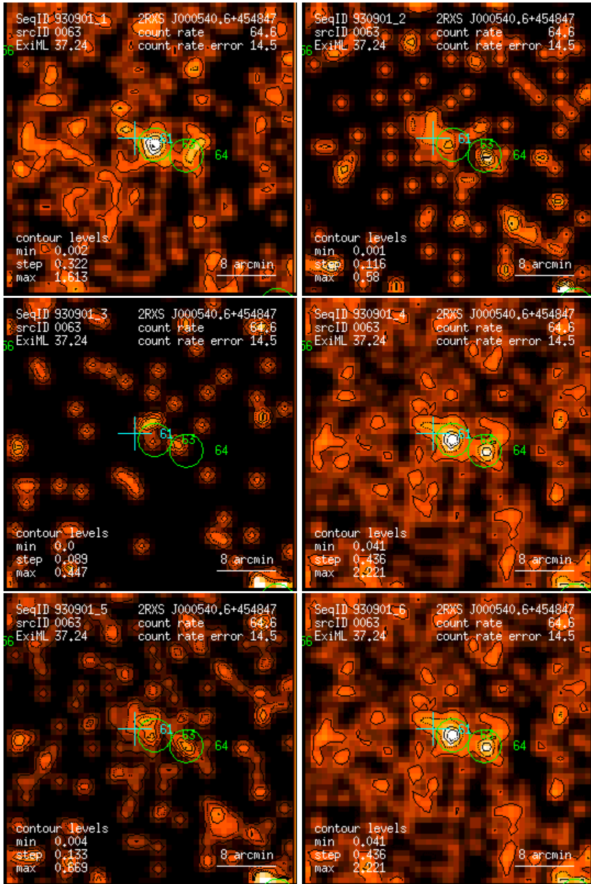
Figure 63: RASS 930901: detection 0063: band rate images, Gaussian filter: (1) PSPC channels 11 – 41, (2) 52 – 90, (3) 91 – 201, (4) 11 – 235, (5) 52 – 201, (6) 11 – 201. Broad band rates in counts/ks. Band rate contour levels in counts/ks/arcmin 2 .
