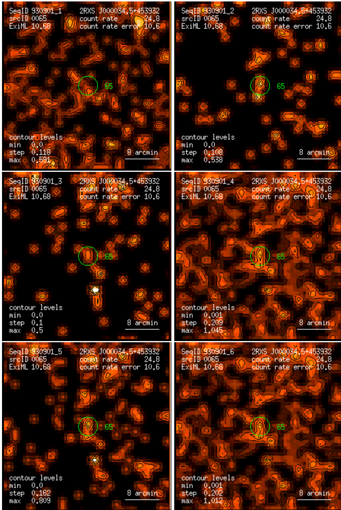
Figure 65: RASS 930901: detection 0065: band rate images, Gaussian filter: (1) PSPC channels 11 – 41, (2) 52 – 90, (3) 91 – 201, (4) 11 – 235, (5) 52 – 201, (6) 11 – 201. Broad band rates in counts/ks. Band rate contour levels in counts/ks/arcmin 2 .
