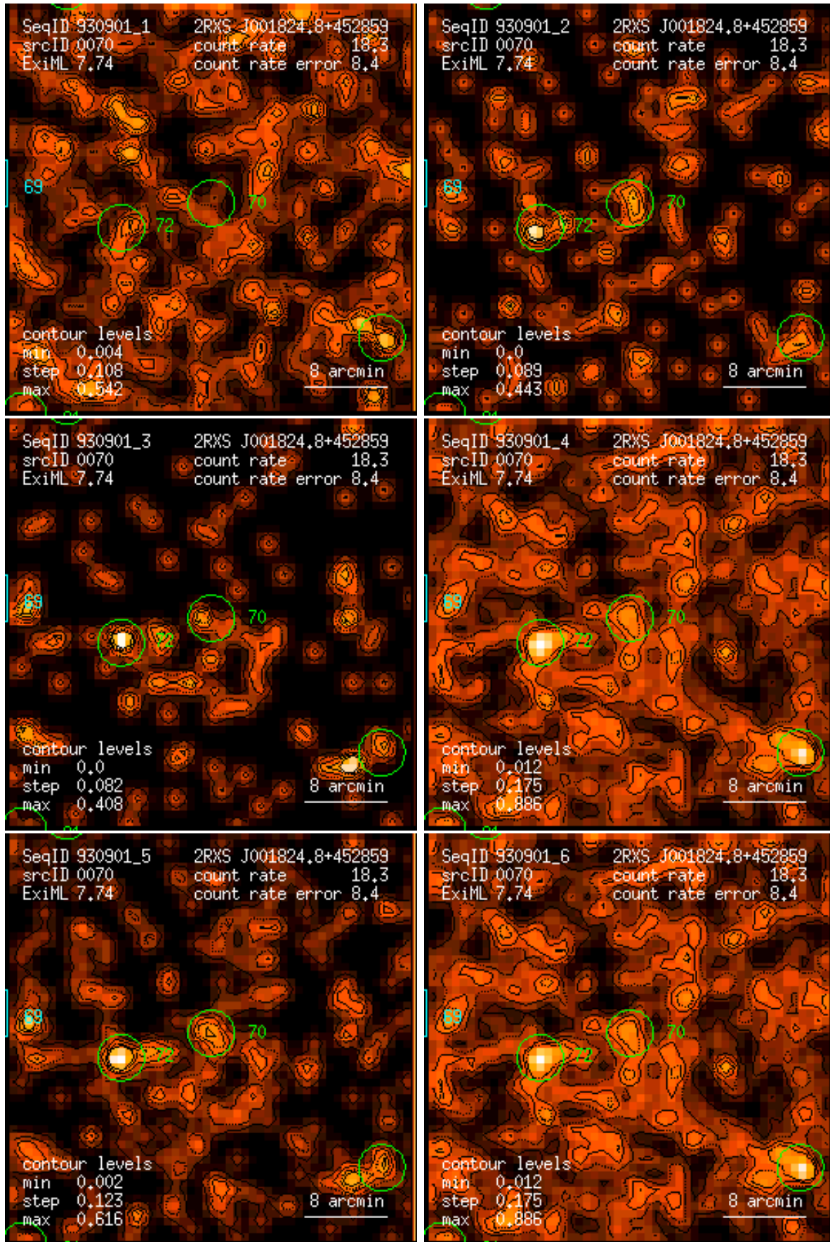
Figure 70: RASS 930901: detection 0070: band rate images, Gaussian filter: (1) PSPC channels 11 – 41, (2) 52 – 90, (3) 91 – 201, (4) 11 – 235, (5) 52 – 201, (6) 11 – 201. Broad band rates in counts/ks. Band rate contour levels in counts/ks/arcmin 2 .
