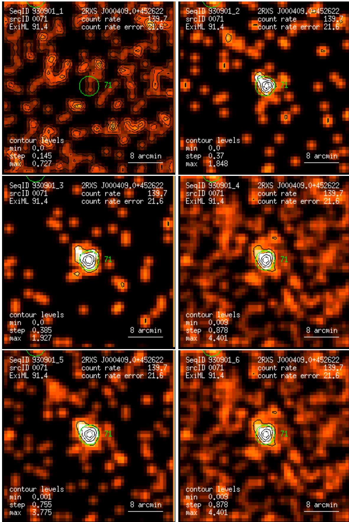
Figure 71: RASS 930901: detection 0071: band rate images, Gaussian filter: (1) PSPC channels 11 – 41, (2) 52 – 90, (3) 91 – 201, (4) 11 – 235, (5) 52 – 201, (6) 11 – 201. Broad band rates in counts/ks. Band rate contour levels in counts/ks/arcmin 2 .
