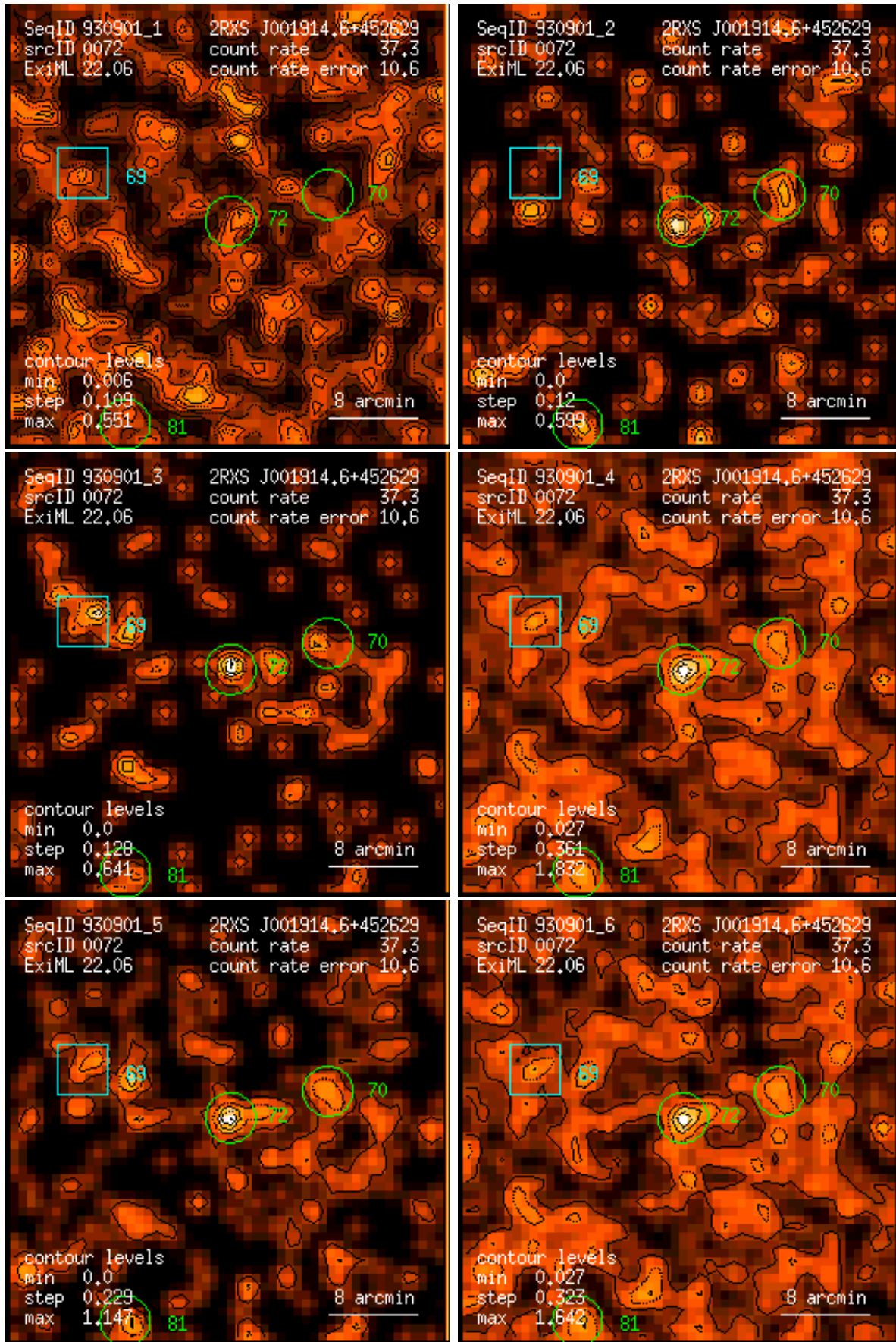
Figure 72: RASS 930901: detection 0072: band rate images, Gaussian filter: (1) PSPC channels 11 – 41, (2) 52 – 90, (3) 91 – 201, (4) 11 – 235, (5) 52 – 201, (6) 11 – 201. Broad band rates in counts/ks. Band rate contour levels in counts/ks/arcmin 2 .
