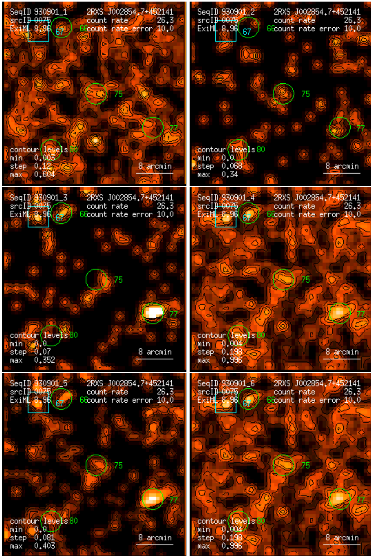
Figure 75: RASS 930901: detection 0075: band rate images, Gaussian filter: (1) PSPC channels 11 – 41, (2) 52 – 90, (3) 91 – 201, (4) 11 – 235, (5) 52 – 201, (6) 11 – 201. Broad band rates in counts/ks. Band rate contour levels in counts/ks/arcmin 2 .
