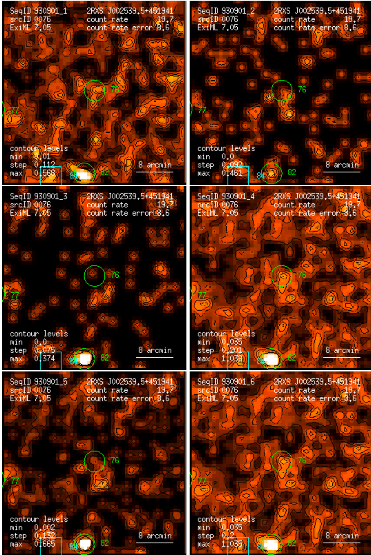
Figure 76: RASS 930901: detection 0076: band rate images, Gaussian filter: (1) PSPC channels 11 – 41, (2) 52 – 90, (3) 91 – 201, (4) 11 – 235, (5) 52 – 201, (6) 11 – 201. Broad band rates in counts/ks. Band rate contour levels in counts/ks/arcmin 2 .
