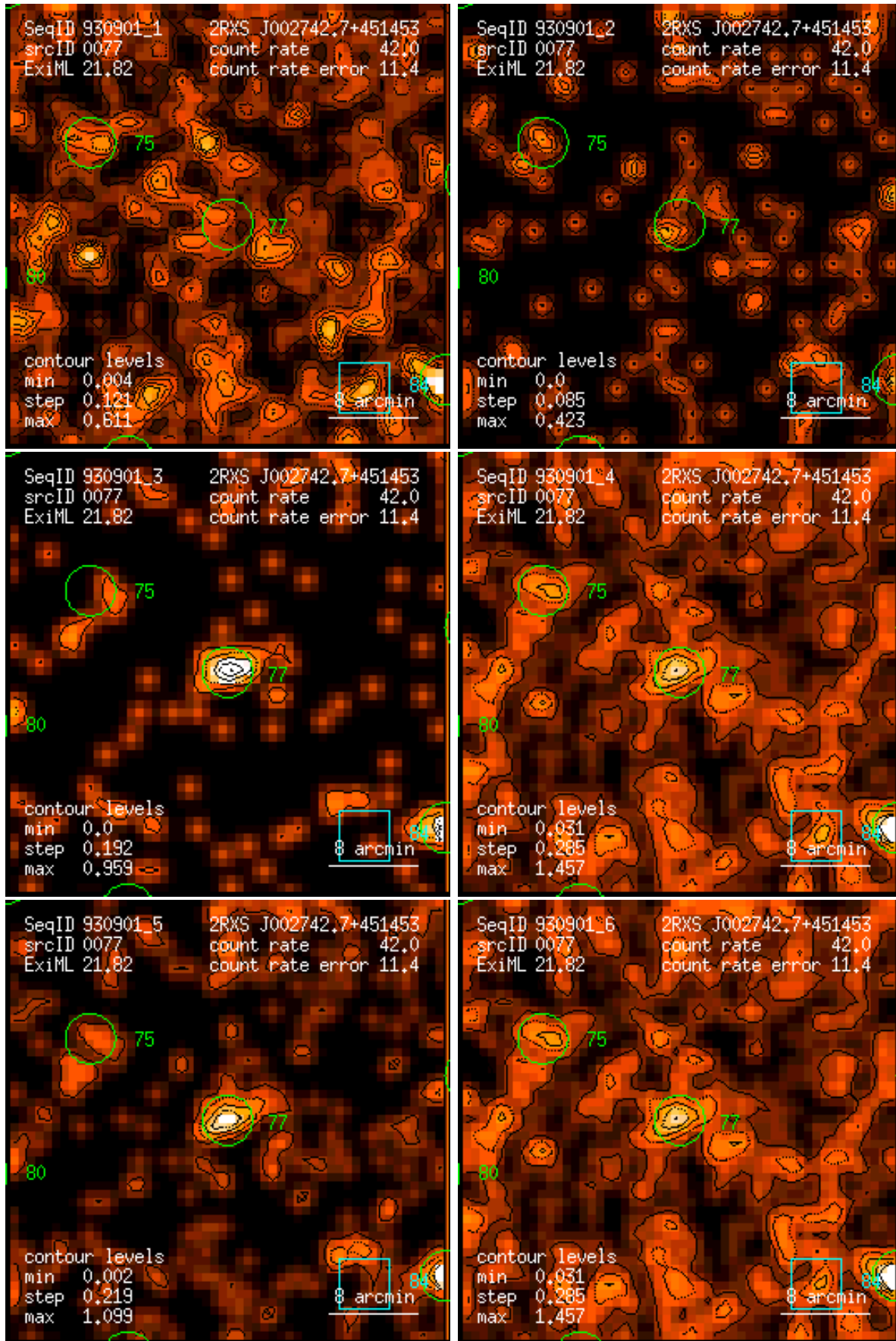
Figure 77: RASS 930901: detection 0077: band rate images, Gaussian filter: (1) PSPC channels 11 – 41, (2) 52 – 90, (3) 91 – 201, (4) 11 – 235, (5) 52 – 201, (6) 11 – 201. Broad band rates in counts/ks. Band rate contour levels in counts/ks/arcmin 2 .
