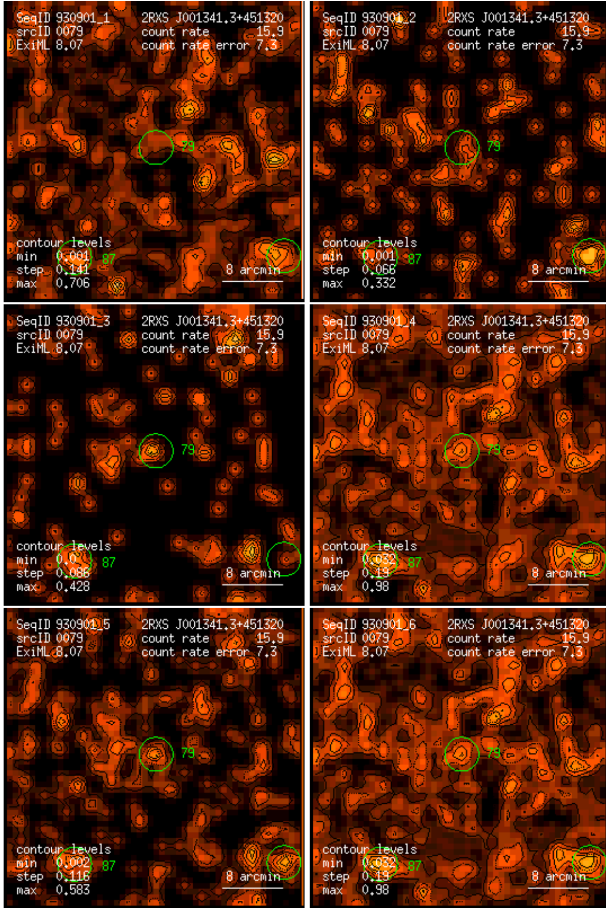
Figure 79: RASS 930901: detection 0079: band rate images, Gaussian filter: (1) PSPC channels 11 – 41, (2) 52 – 90, (3) 91 – 201, (4) 11 – 235, (5) 52 – 201, (6) 11 – 201. Broad band rates in counts/ks. Band rate contour levels in counts/ks/arcmin 2 .
