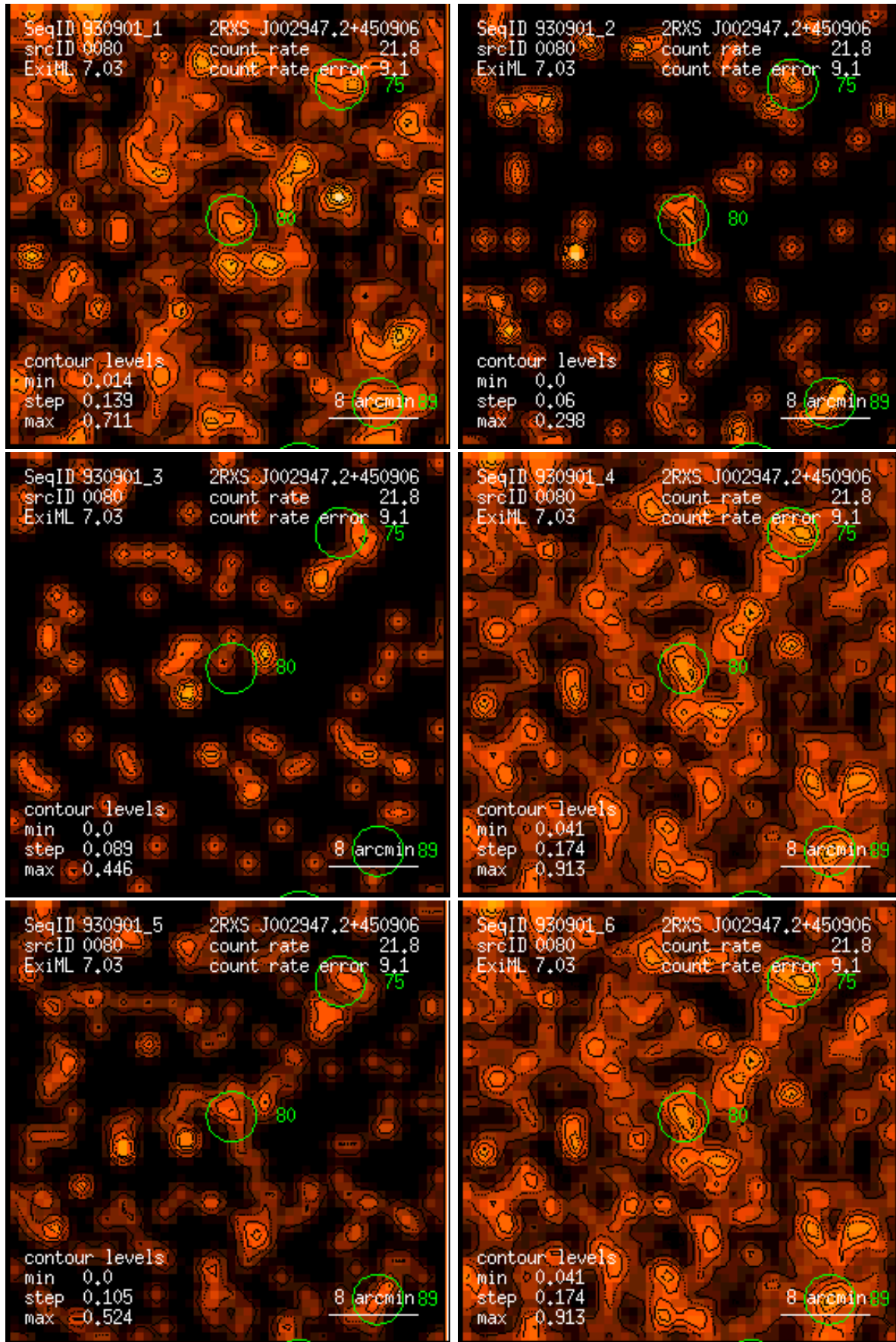
Figure 80: RASS 930901: detection 0080: band rate images, Gaussian filter: (1) PSPC channels 11 – 41, (2) 52 – 90, (3) 91 – 201, (4) 11 – 235, (5) 52 – 201, (6) 11 – 201. Broad band rates in counts/ks. Band rate contour levels in counts/ks/arcmin 2 .
