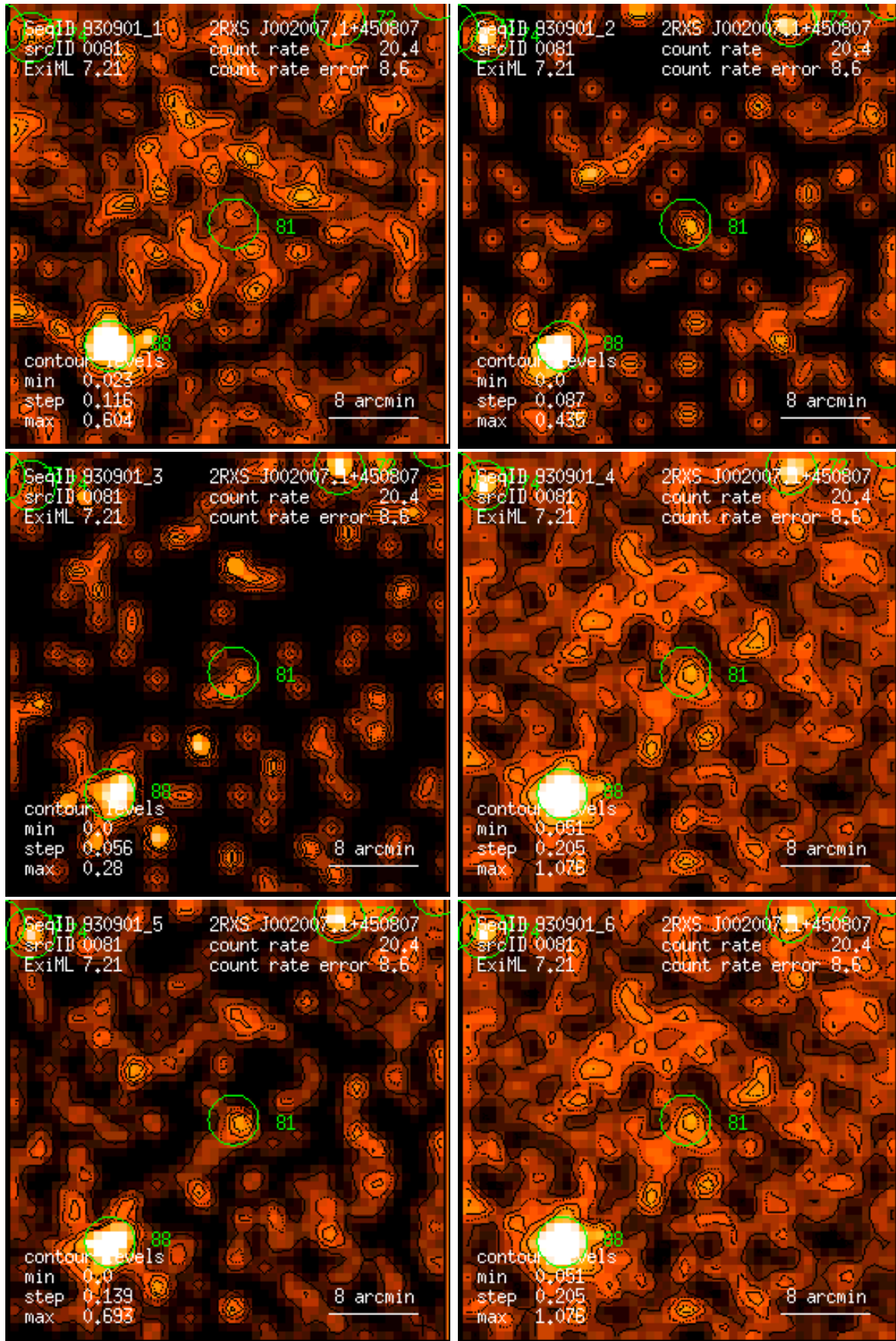
Figure 81: RASS 930901: detection 0081: band rate images, Gaussian filter: (1) PSPC channels 11 – 41, (2) 52 – 90, (3) 91 – 201, (4) 11 – 235, (5) 52 – 201, (6) 11 – 201. Broad band rates in counts/ks. Band rate contour levels in counts/ks/arcmin 2 .
