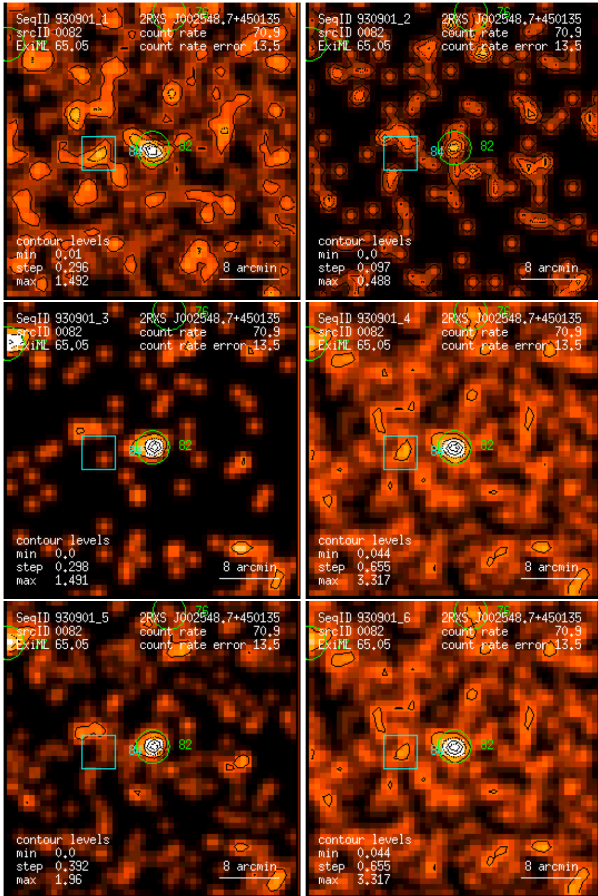
Figure 82: RASS 930901: detection 0082: band rate images, Gaussian filter: (1) PSPC channels 11 – 41, (2) 52 – 90, (3) 91 – 201, (4) 11 – 235, (5) 52 – 201, (6) 11 – 201. Broad band rates in counts/ks. Band rate contour levels in counts/ks/arcmin 2 .
