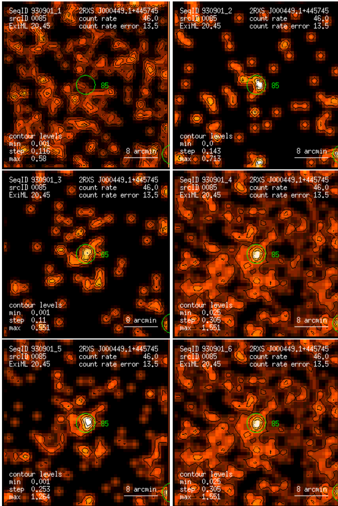
Figure 85: RASS 930901: detection 0085: band rate images, Gaussian filter: (1) PSPC channels 11 – 41, (2) 52 – 90, (3) 91 – 201, (4) 11 – 235, (5) 52 – 201, (6) 11 – 201. Broad band rates in counts/ks. Band rate contour levels in counts/ks/arcmin 2 .
