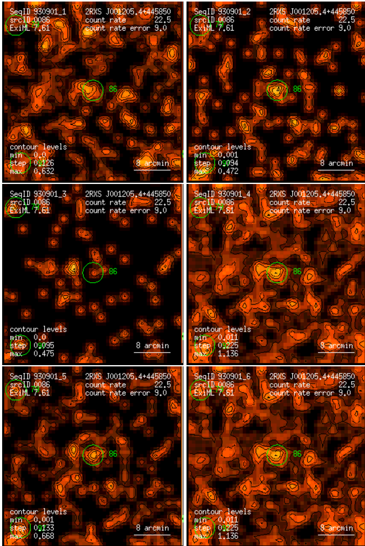
Figure 86: RASS 930901: detection 0086: band rate images, Gaussian filter: (1) PSPC channels 11 – 41, (2) 52 – 90, (3) 91 – 201, (4) 11 – 235, (5) 52 – 201, (6) 11 – 201. Broad band rates in counts/ks. Band rate contour levels in counts/ks/arcmin 2 .
