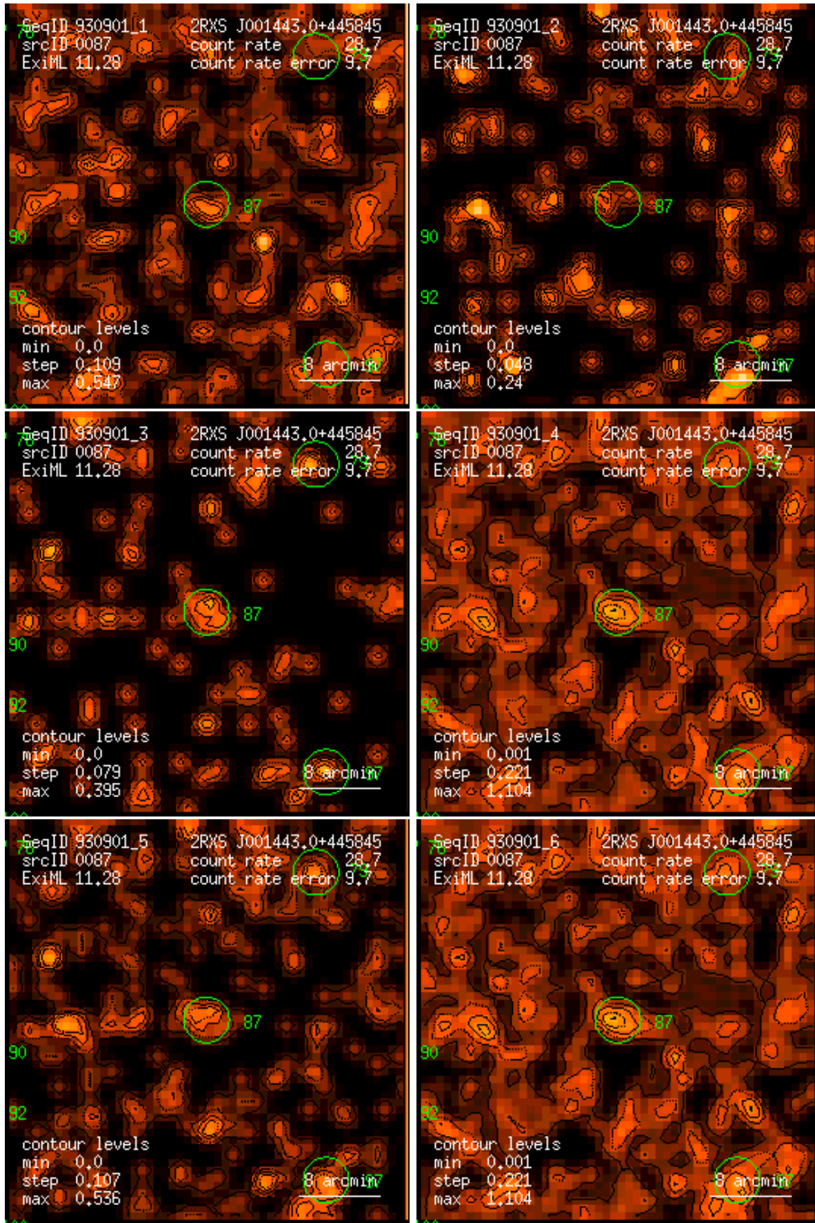
Figure 87: RASS 930901: detection 0087: band rate images, Gaussian filter: (1) PSPC channels 11 – 41, (2) 52 – 90, (3) 91 – 201, (4) 11 – 235, (5) 52 – 201, (6) 11 – 201. Broad band rates in counts/ks. Band rate contour levels in counts/ks/arcmin 2 .
