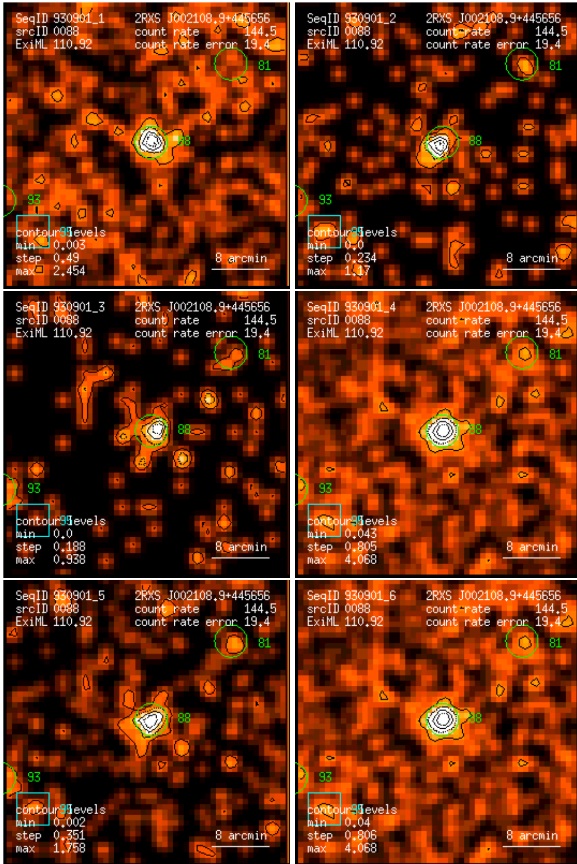
Figure 88: RASS 930901: detection 0088: band rate images, Gaussian filter: (1) PSPC channels 11 – 41, (2) 52 – 90, (3) 91 – 201, (4) 11 – 235, (5) 52 – 201, (6) 11 – 201. Broad band rates in counts/ks. Band rate contour levels in counts/ks/arcmin 2 .
